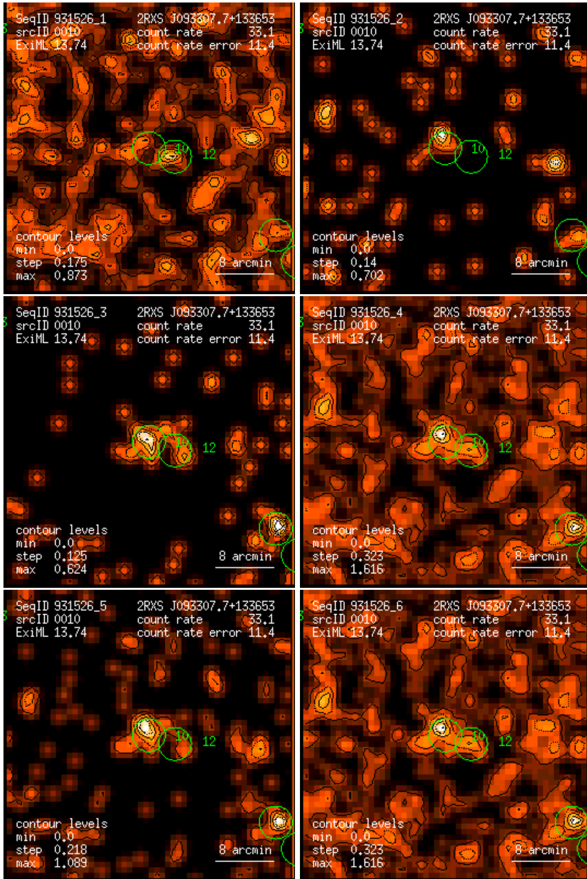
Figure 10: RASS 931526: detection 0010: band rate images, Gaussian filter: (1) PSPC channels 11 – 41, (2) 52 – 90, (3) 91 – 201, (4) 11 – 235, (5) 52 – 201, (6) 11 – 201. Broad band rates in counts/ks. Band rate contour levels in counts/ks/arcmin 2 .
