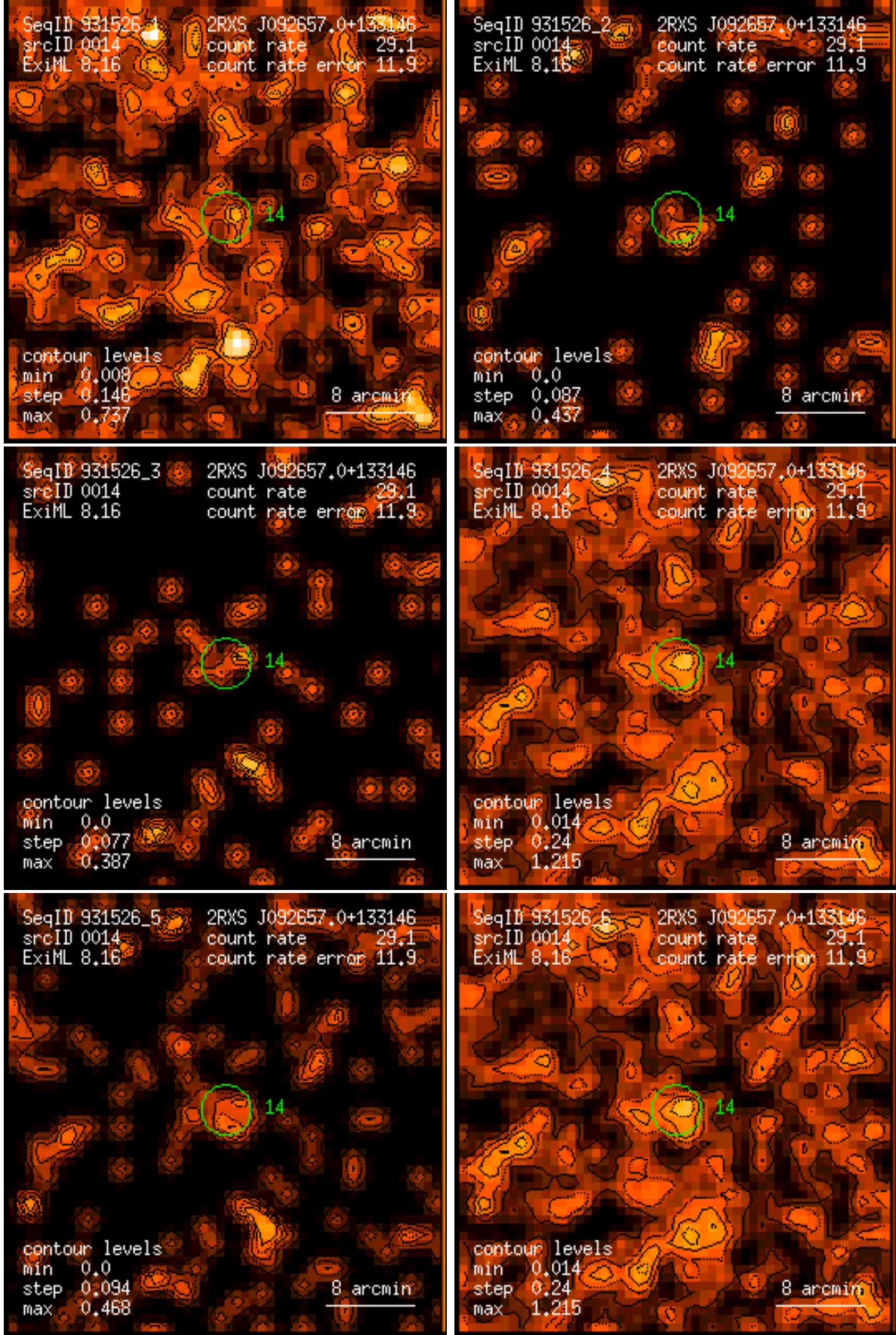
Figure 14: RASS 931526: detection 0014: band rate images, Gaussian filter: (1) PSPC channels 11 – 41, (2) 52 – 90, (3) 91 – 201, (4) 11 – 235, (5) 52 – 201, (6) 11 – 201. Broad band rates in counts/ks. Band rate contour levels in counts/ks/arcmin 2 .
