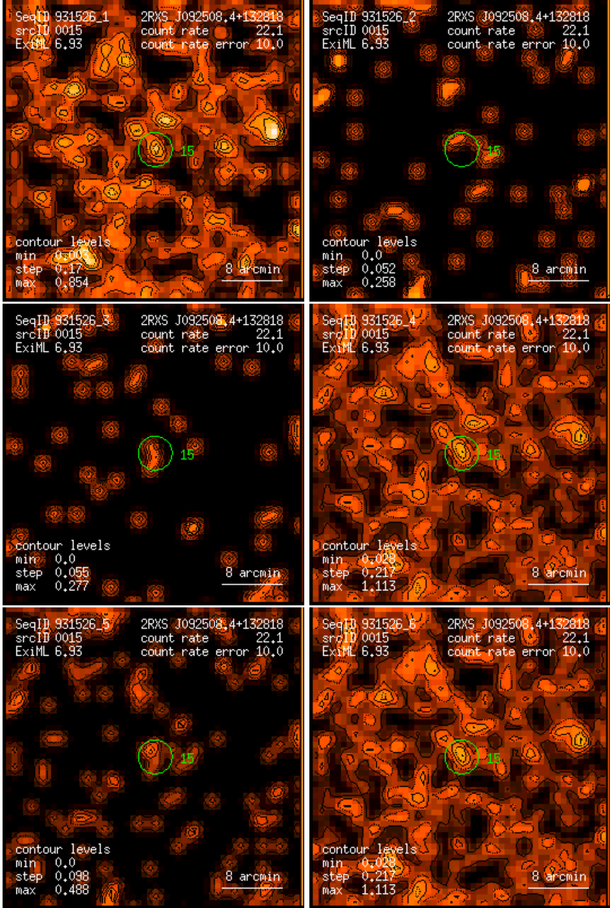
Figure 15: RASS 931526: detection 0015: band rate images, Gaussian filter: (1) PSPC channels 11 – 41, (2) 52 – 90, (3) 91 – 201, (4) 11 – 235, (5) 52 – 201, (6) 11 – 201. Broad band rates in counts/ks. Band rate contour levels in counts/ks/arcmin 2 .
