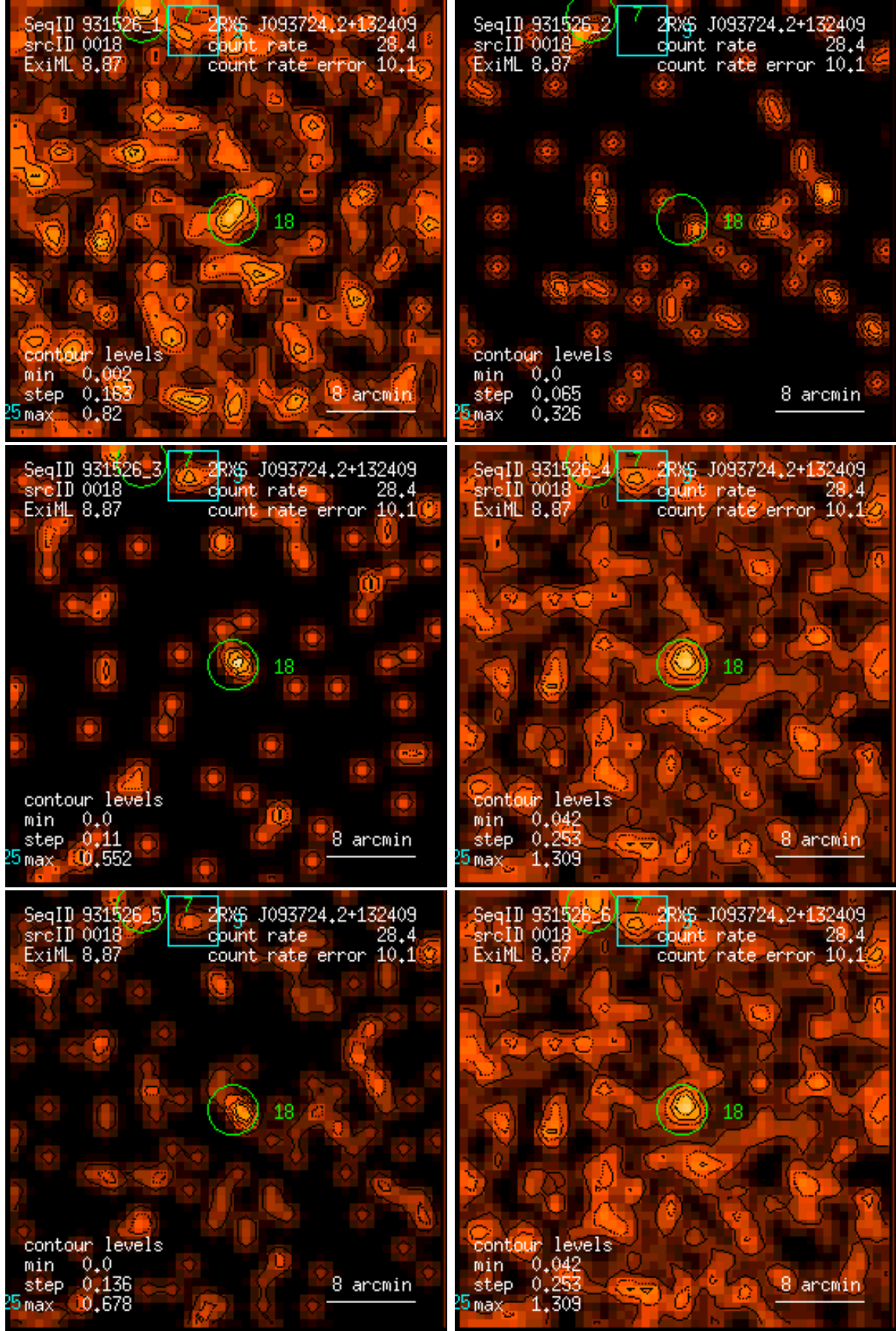
Figure 18: RASS 931526: detection 0018: band rate images, Gaussian filter: (1) PSPC channels 11 – 41, (2) 52 – 90, (3) 91 – 201, (4) 11 – 235, (5) 52 – 201, (6) 11 – 201. Broad band rates in counts/ks. Band rate contour levels in counts/ks/arcmin 2 .
