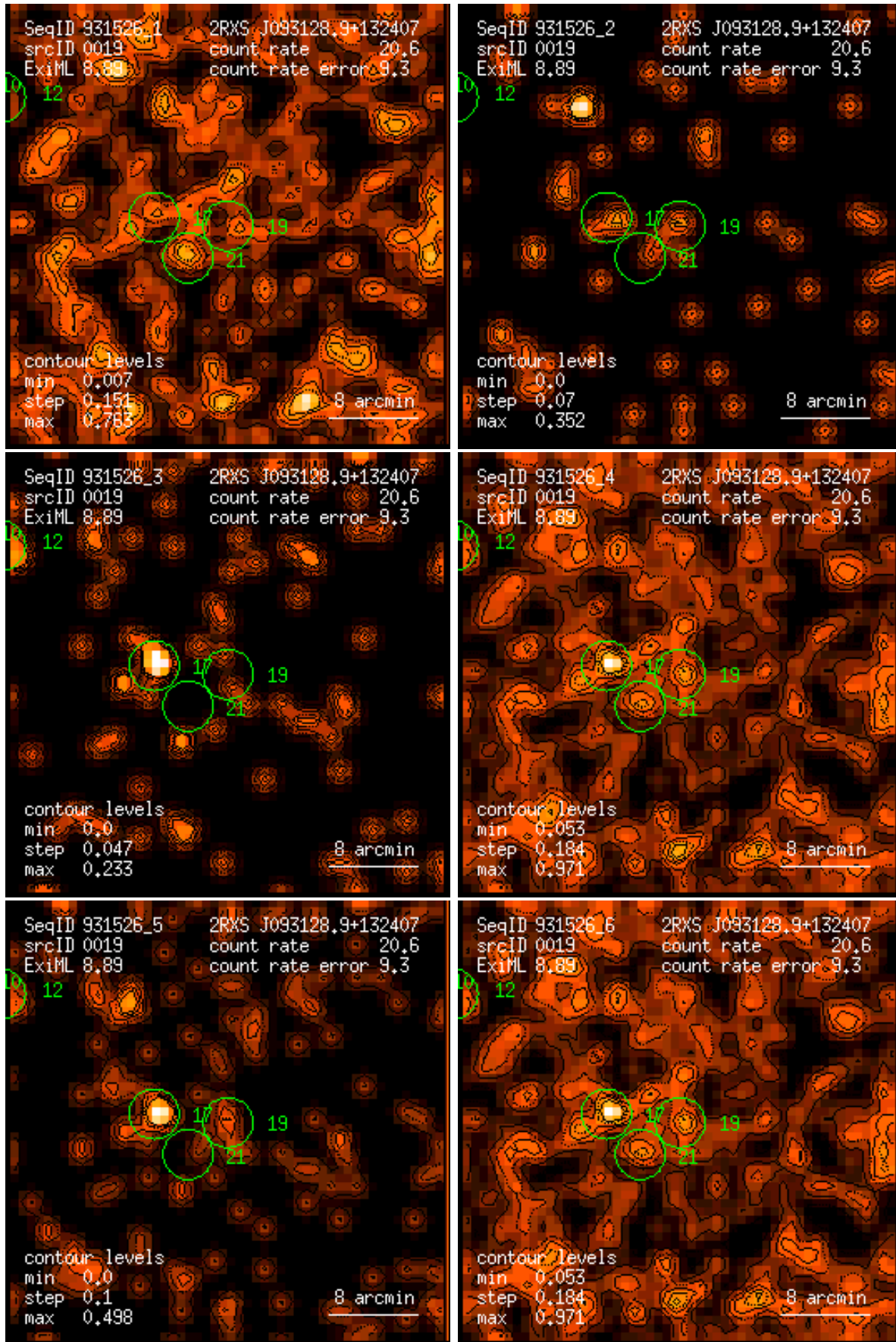
Figure 19: RASS 931526: detection 0019: band rate images, Gaussian filter: (1) PSPC channels 11 – 41, (2) 52 – 90, (3) 91 – 201, (4) 11 – 235, (5) 52 – 201, (6) 11 – 201. Broad band rates in counts/ks. Band rate contour levels in counts/ks/arcmin 2 .
