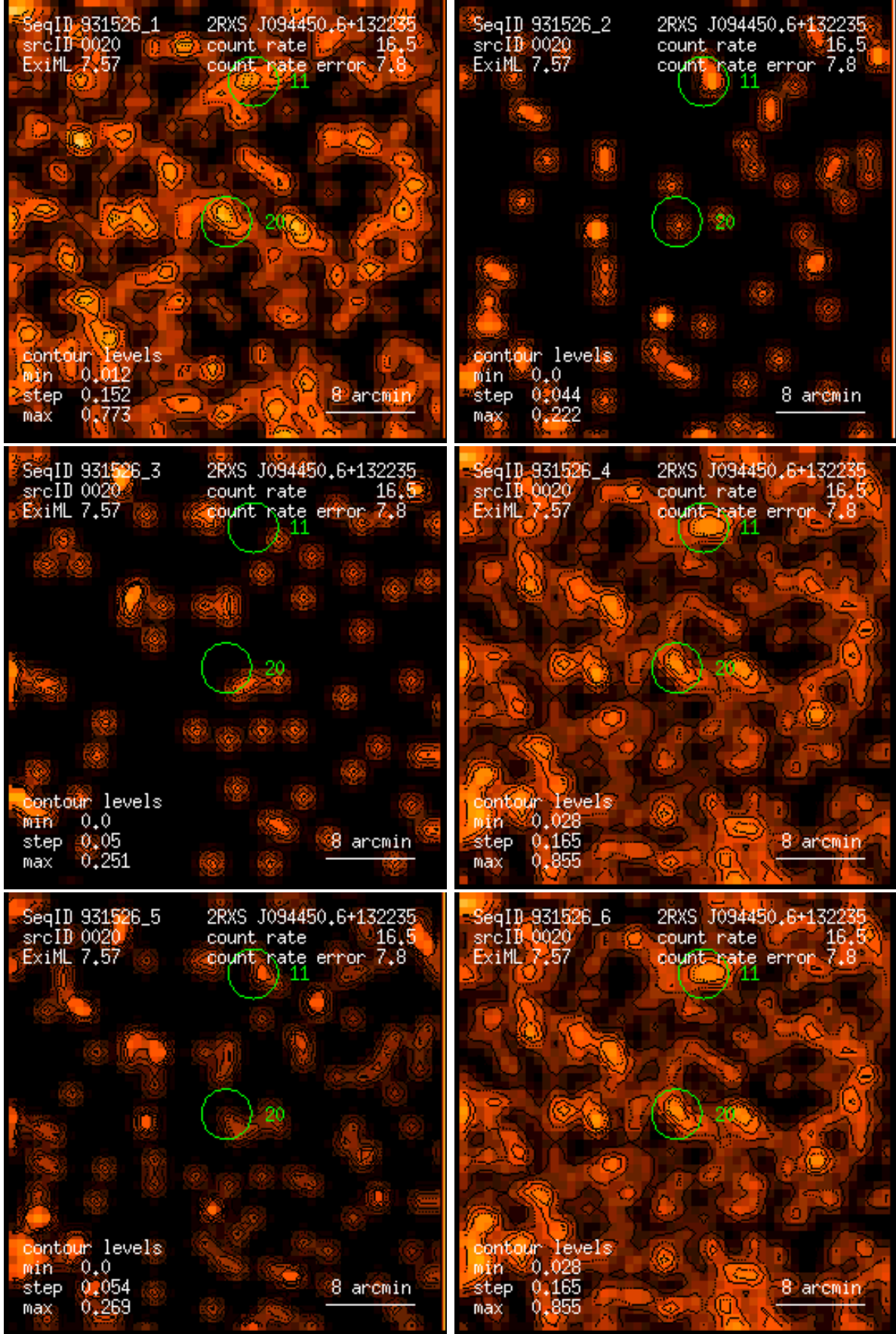
Figure 20: RASS 931526: detection 0020: band rate images, Gaussian filter: (1) PSPC channels 11 – 41, (2) 52 – 90, (3) 91 – 201, (4) 11 – 235, (5) 52 – 201, (6) 11 – 201. Broad band rates in counts/ks. Band rate contour levels in counts/ks/arcmin 2 .
