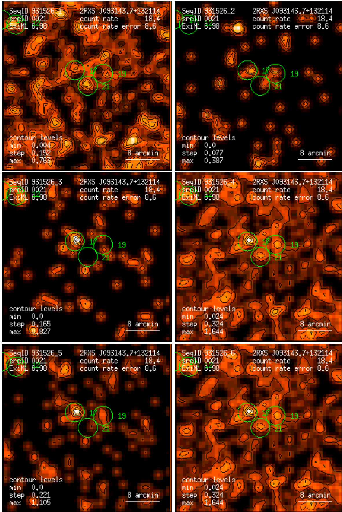
Figure 21: RASS 931526: detection 0021: band rate images, Gaussian filter: (1) PSPC channels 11 – 41, (2) 52 – 90, (3) 91 – 201, (4) 11 – 235, (5) 52 – 201, (6) 11 – 201. Broad band rates in counts/ks. Band rate contour levels in counts/ks/arcmin 2 .
