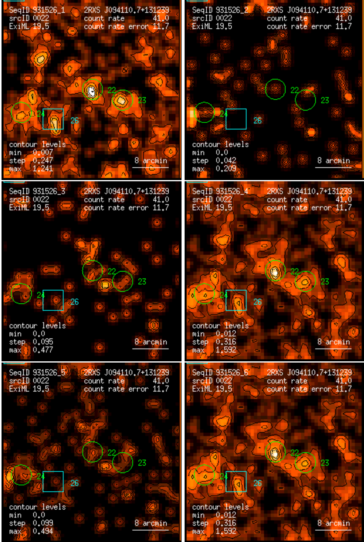
Figure 22: RASS 931526: detection 0022: band rate images, Gaussian filter: (1) PSPC channels 11 – 41, (2) 52 – 90, (3) 91 – 201, (4) 11 – 235, (5) 52 – 201, (6) 11 – 201. Broad band rates in counts/ks. Band rate contour levels in counts/ks/arcmin 2 .
