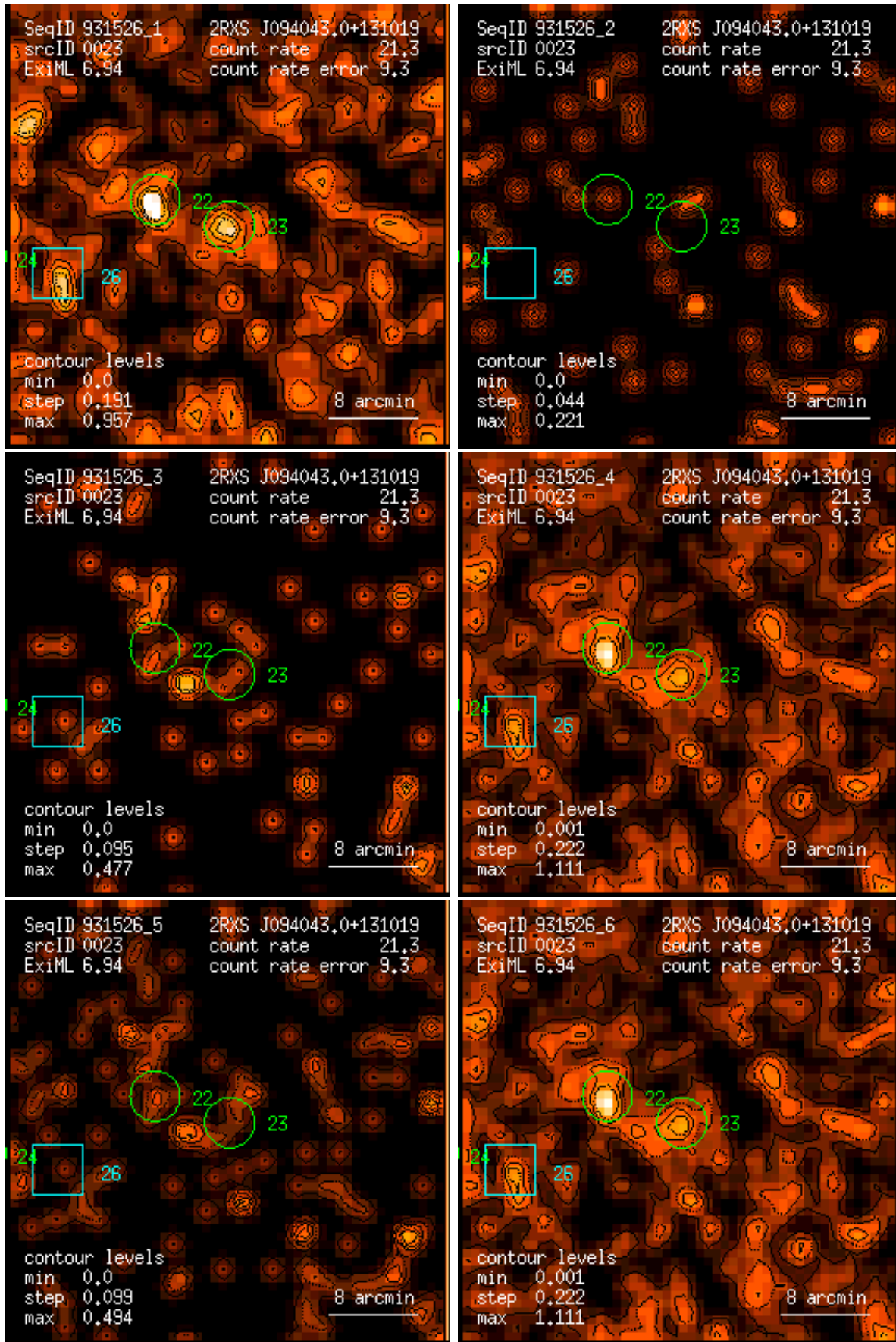
Figure 23: RASS 931526: detection 0023: band rate images, Gaussian filter: (1) PSPC channels 11 – 41, (2) 52 – 90, (3) 91 – 201, (4) 11 – 235, (5) 52 – 201, (6) 11 – 201. Broad band rates in counts/ks. Band rate contour levels in counts/ks/arcmin 2 .
