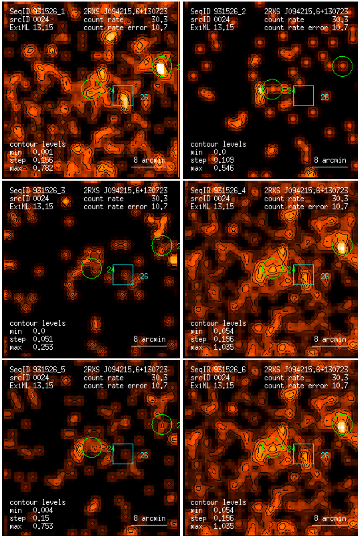
Figure 24: RASS 931526: detection 0024: band rate images, Gaussian filter: (1) PSPC channels 11 – 41, (2) 52 – 90, (3) 91 – 201, (4) 11 – 235, (5) 52 – 201, (6) 11 – 201. Broad band rates in counts/ks. Band rate contour levels in counts/ks/arcmin 2 .
