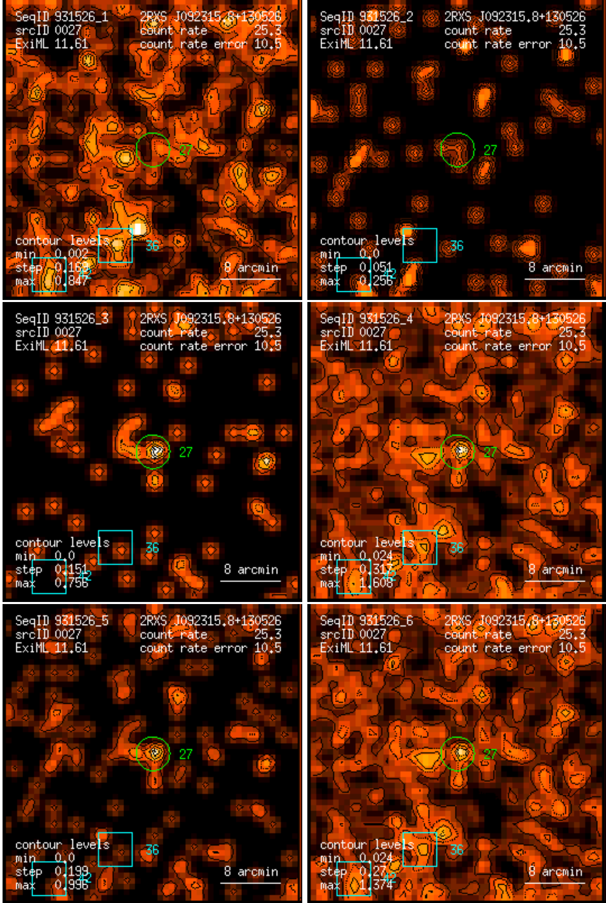
Figure 27: RASS 931526: detection 0027: band rate images, Gaussian filter: (1) PSPC channels 11 – 41, (2) 52 – 90, (3) 91 – 201, (4) 11 – 235, (5) 52 – 201, (6) 11 – 201. Broad band rates in counts/ks. Band rate contour levels in counts/ks/arcmin 2 .
