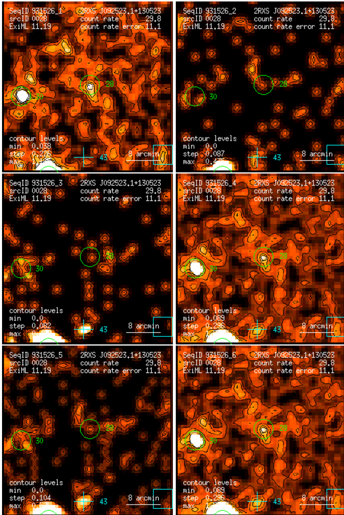
Figure 28: RASS 931526: detection 0028: band rate images, Gaussian filter: (1) PSPC channels 11 – 41, (2) 52 – 90, (3) 91 – 201, (4) 11 – 235, (5) 52 – 201, (6) 11 – 201. Broad band rates in counts/ks. Band rate contour levels in counts/ks/arcmin 2 .
