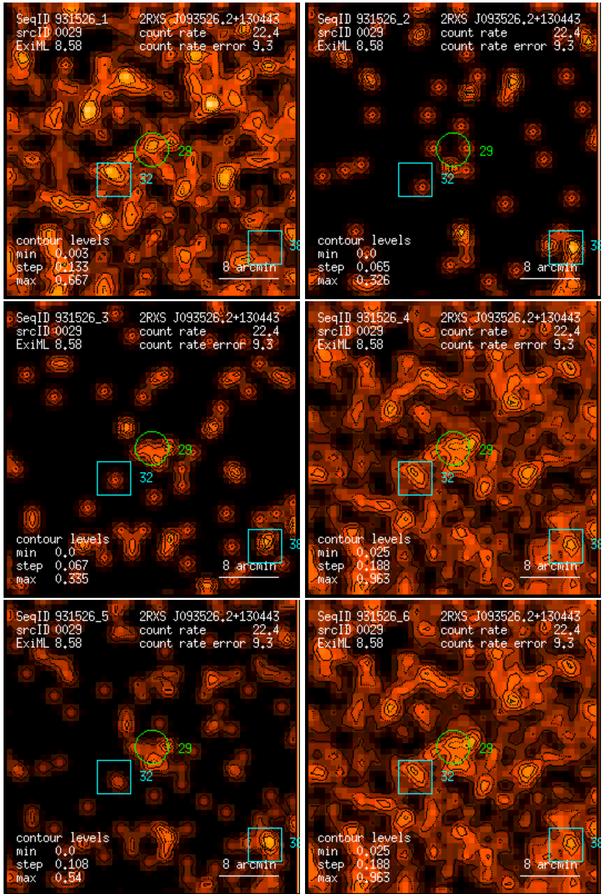
Figure 29: RASS 931526: detection 0029: band rate images, Gaussian filter: (1) PSPC channels 11 – 41, (2) 52 – 90, (3) 91 – 201, (4) 11 – 235, (5) 52 – 201, (6) 11 – 201. Broad band rates in counts/ks. Band rate contour levels in counts/ks/arcmin 2 .
