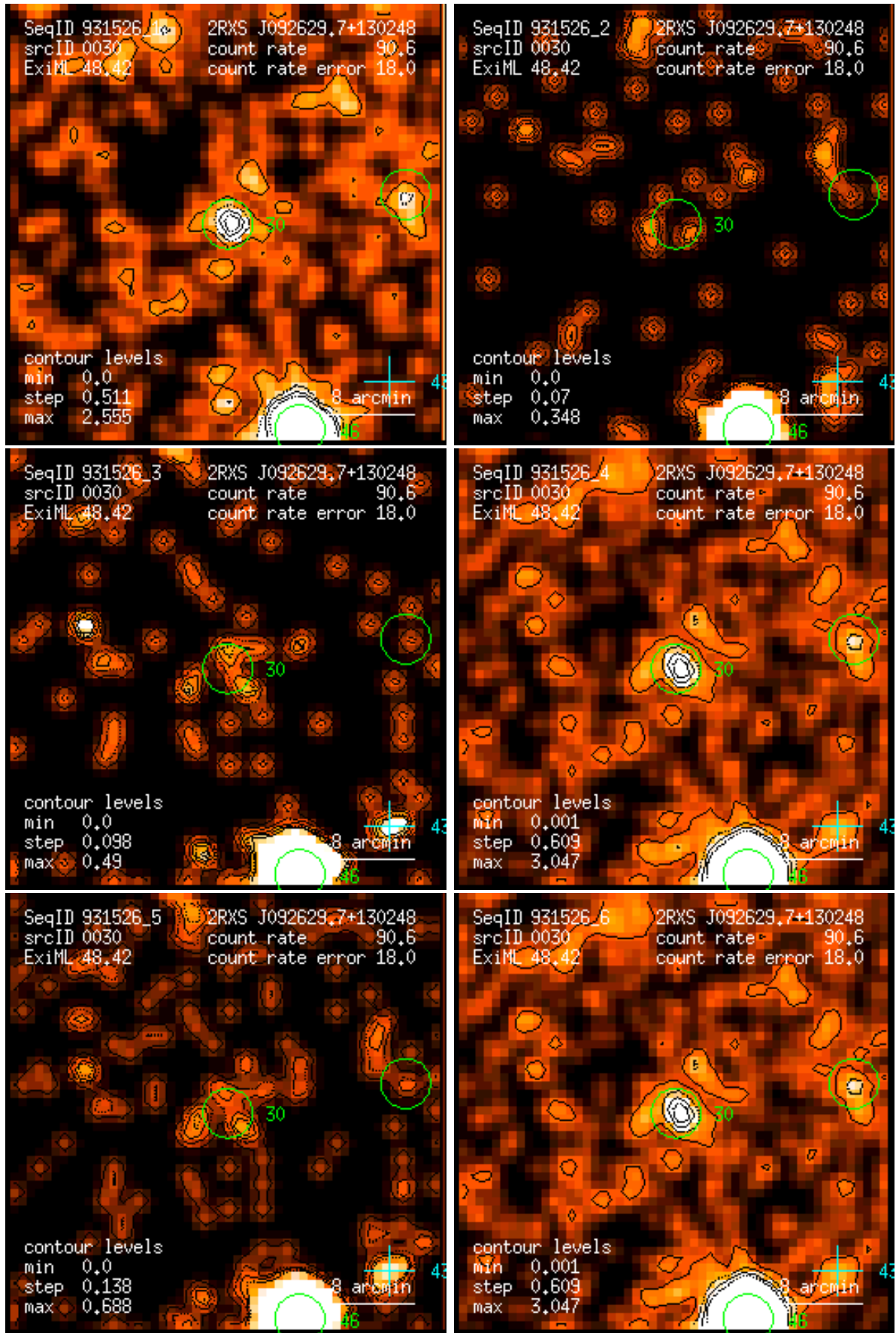
Figure 30: RASS 931526: detection 0030: band rate images, Gaussian filter: (1) PSPC channels 11 – 41, (2) 52 – 90, (3) 91 – 201, (4) 11 – 235, (5) 52 – 201, (6) 11 – 201. Broad band rates in counts/ks. Band rate contour levels in counts/ks/arcmin 2 .
