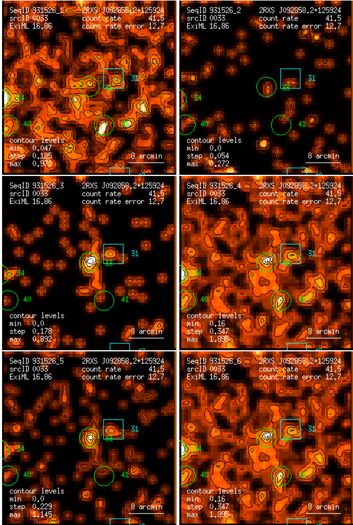
Figure 33: RASS 931526: detection 0033: band rate images, Gaussian filter: (1) PSPC channels 11 – 41, (2) 52 – 90, (3) 91 – 201, (4) 11 – 235, (5) 52 – 201, (6) 11 – 201. Broad band rates in counts/ks. Band rate contour levels in counts/ks/arcmin 2 .
