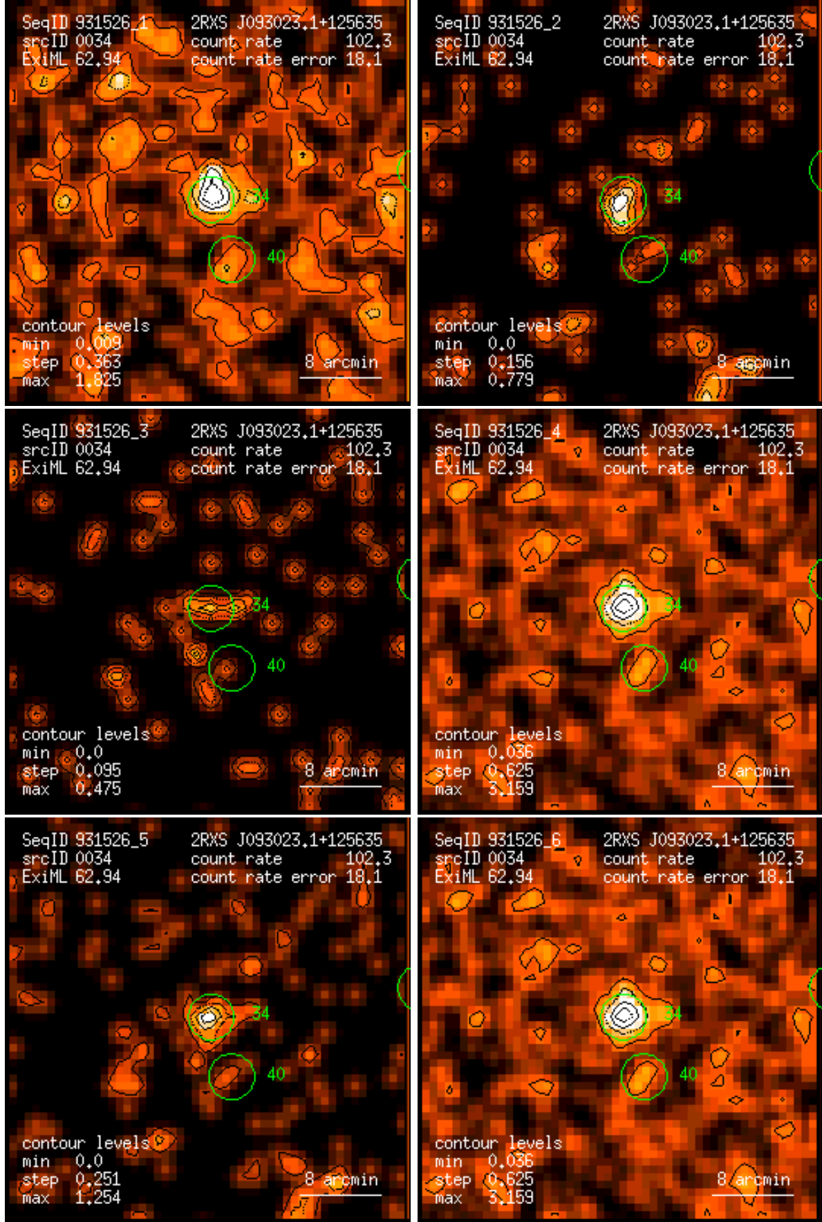
Figure 34: RASS 931526: detection 0034: band rate images, Gaussian filter: (1) PSPC channels 11 – 41, (2) 52 – 90, (3) 91 – 201, (4) 11 – 235, (5) 52 – 201, (6) 11 – 201. Broad band rates in counts/ks. Band rate contour levels in counts/ks/arcmin 2 .
