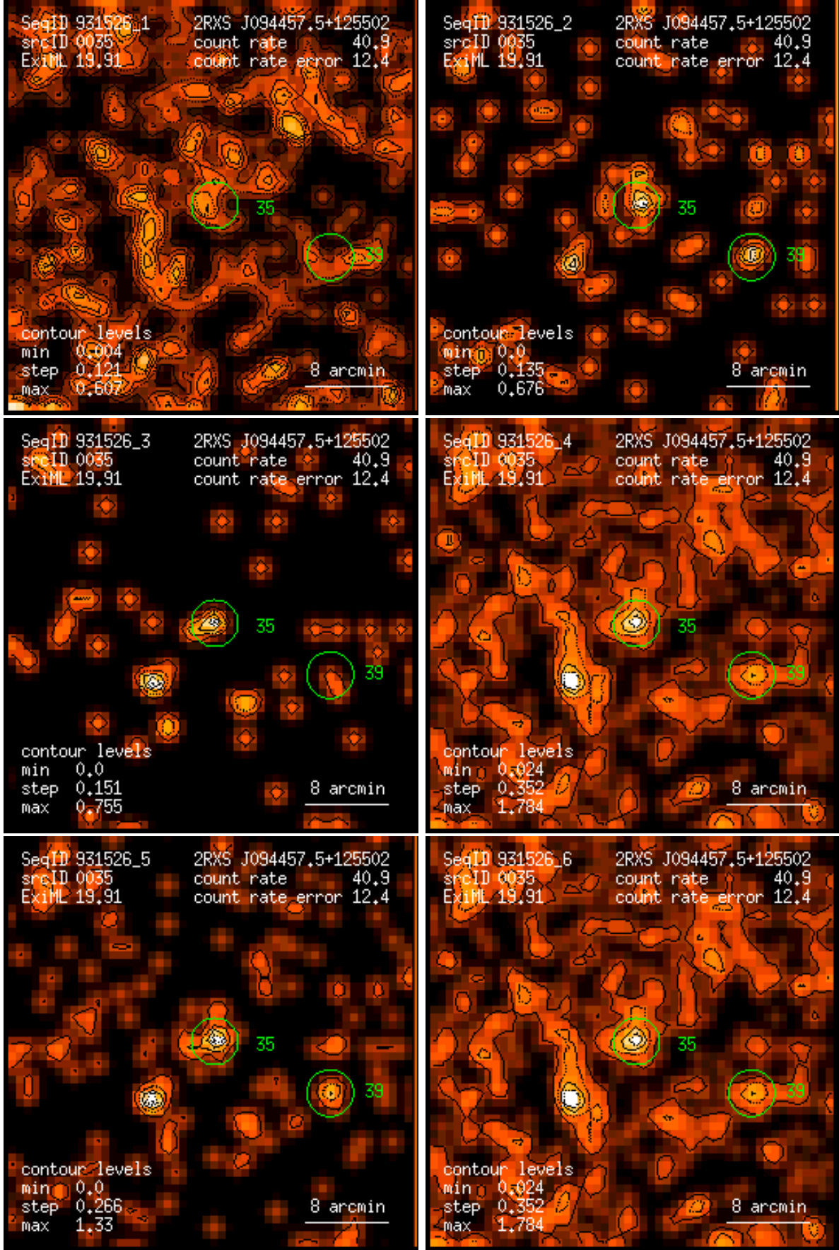
Figure 35: RASS 931526: detection 0035: band rate images, Gaussian filter: (1) PSPC channels 11 – 41, (2) 52 – 90, (3) 91 – 201, (4) 11 – 235, (5) 52 – 201, (6) 11 – 201. Broad band rates in counts/ks. Band rate contour levels in counts/ks/arcmin 2 .
