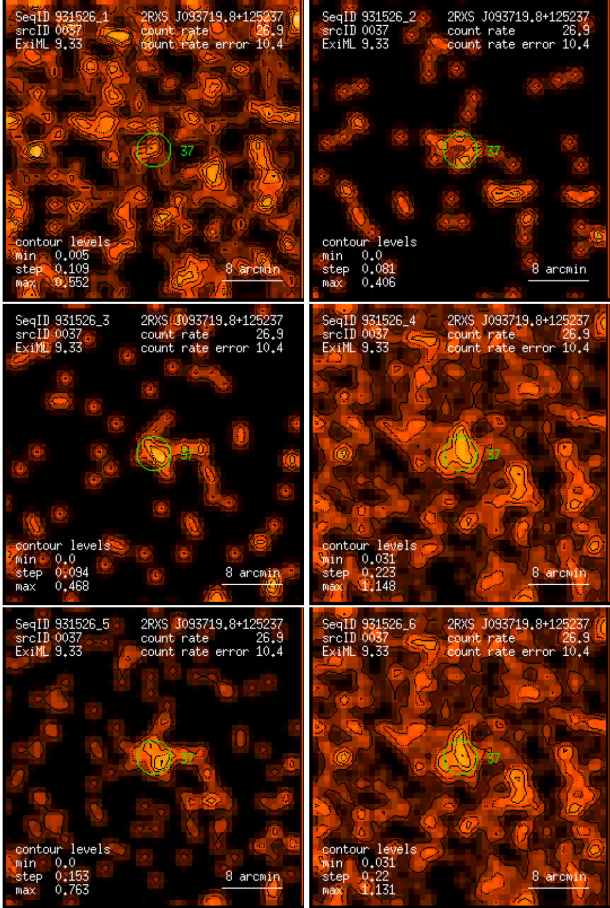
Figure 37: RASS 931526: detection 0037: band rate images, Gaussian filter: (1) PSPC channels 11 – 41, (2) 52 – 90, (3) 91 – 201, (4) 11 – 235, (5) 52 – 201, (6) 11 – 201. Broad band rates in counts/ks. Band rate contour levels in counts/ks/arcmin 2 .
