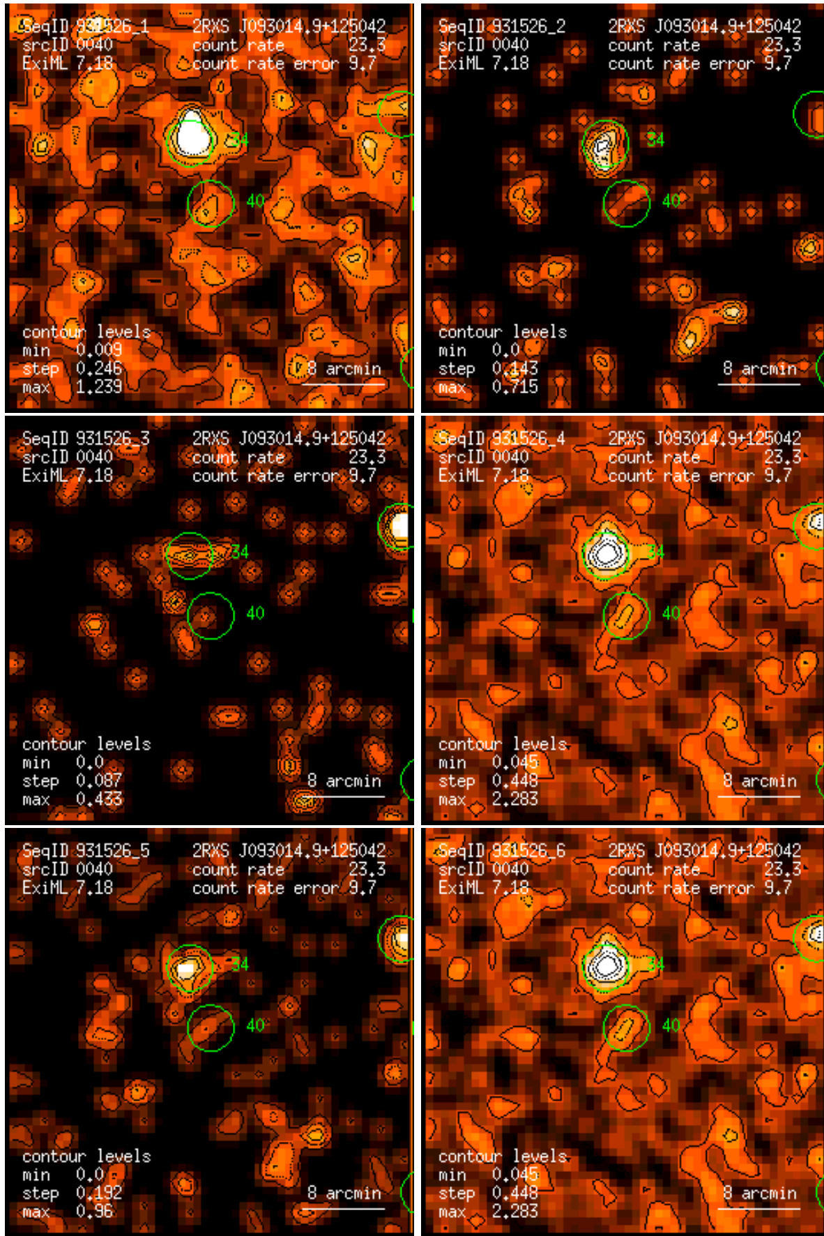
Figure 40: RASS 931526: detection 0040: band rate images, Gaussian filter: (1) PSPC channels 11 – 41, (2) 52 – 90, (3) 91 – 201, (4) 11 – 235, (5) 52 – 201, (6) 11 – 201. Broad band rates in counts/ks. Band rate contour levels in counts/ks/arcmin 2 .
