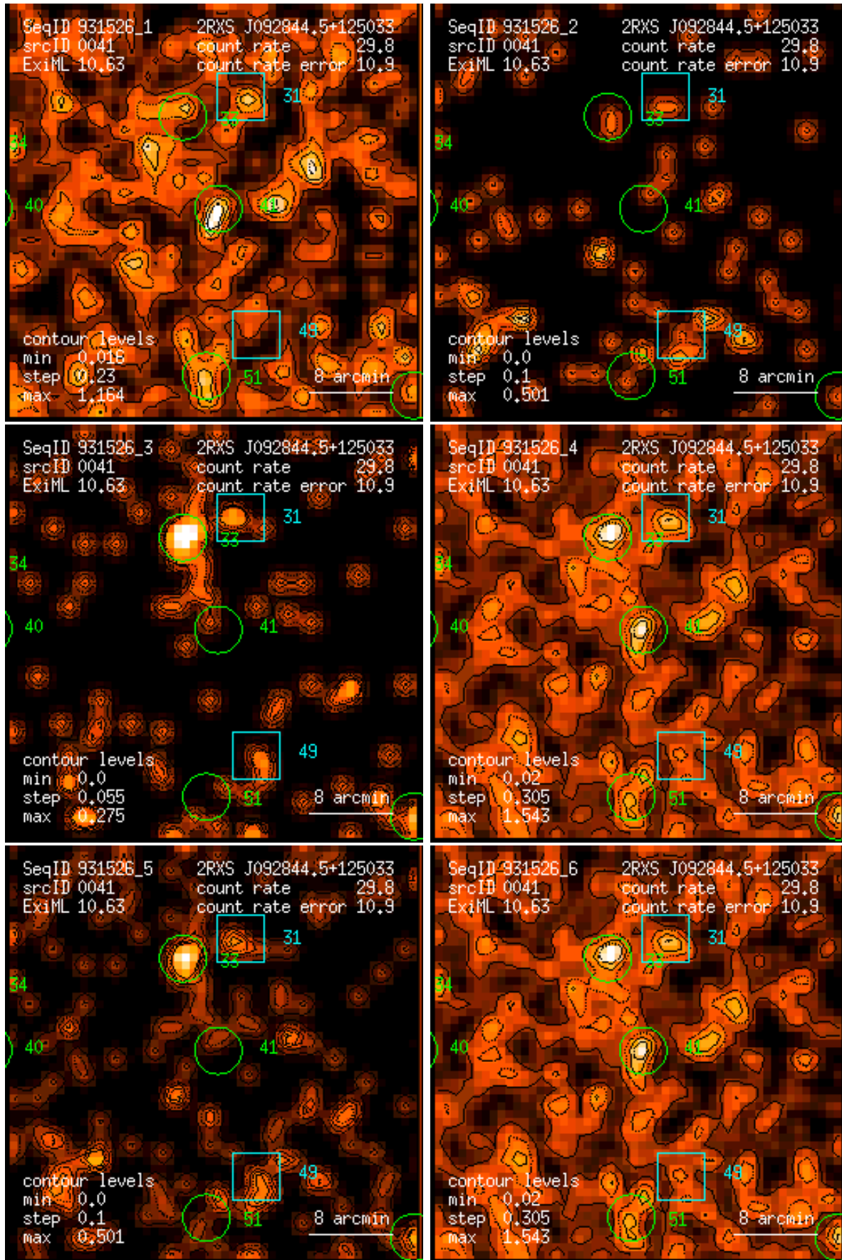
Figure 41: RASS 931526: detection 0041: band rate images, Gaussian filter: (1) PSPC channels 11 – 41, (2) 52 – 90, (3) 91 – 201, (4) 11 – 235, (5) 52 – 201, (6) 11 – 201. Broad band rates in counts/ks. Band rate contour levels in counts/ks/arcmin 2 .
