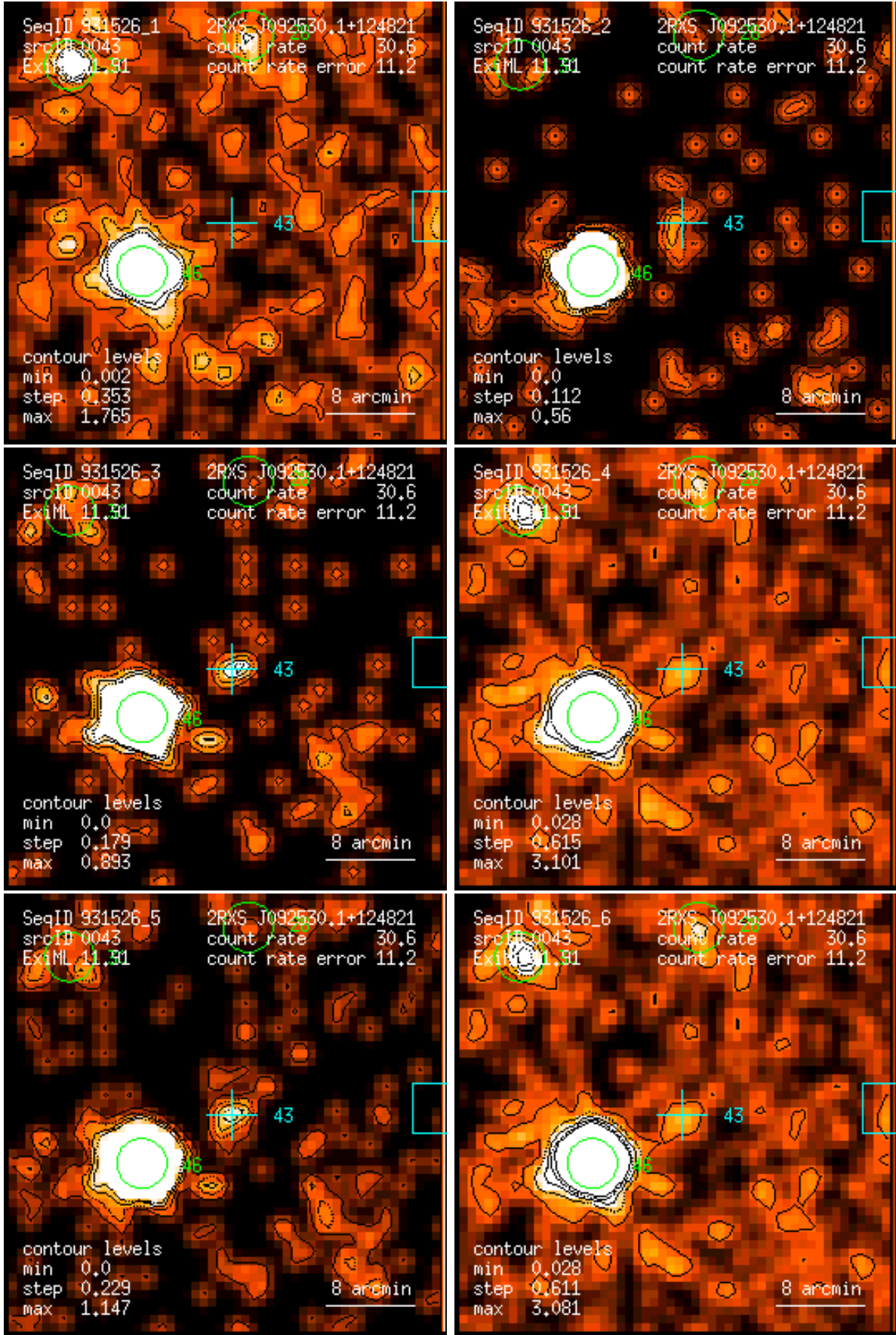
Figure 43: RASS 931526: detection 0043: band rate images, Gaussian filter: (1) PSPC channels 11 – 41, (2) 52 – 90, (3) 91 – 201, (4) 11 – 235, (5) 52 – 201, (6) 11 – 201. Broad band rates in counts/ks. Band rate contour levels in counts/ks/arcmin 2 .
