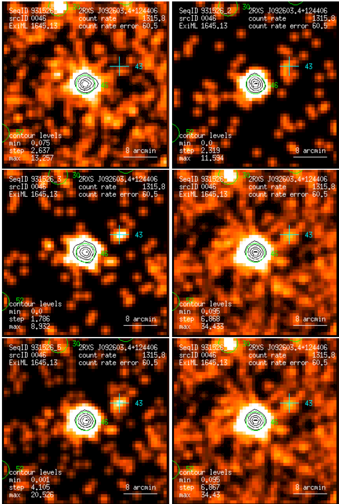
Figure 46: RASS 931526: detection 0046: band rate images, Gaussian filter: (1) PSPC channels 11 – 41, (2) 52 – 90, (3) 91 – 201, (4) 11 – 235, (5) 52 – 201, (6) 11 – 201. Broad band rates in counts/ks. Band rate contour levels in counts/ks/arcmin 2 .
