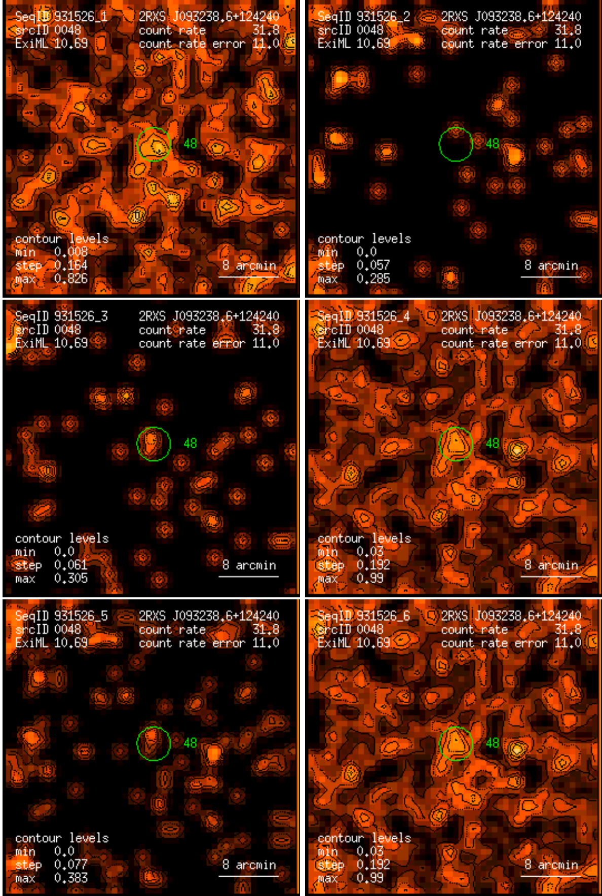
Figure 48: RASS 931526: detection 0048: band rate images, Gaussian filter: (1) PSPC channels 11 – 41, (2) 52 – 90, (3) 91 – 201, (4) 11 – 235, (5) 52 – 201, (6) 11 – 201. Broad band rates in counts/ks. Band rate contour levels in counts/ks/arcmin 2 .
