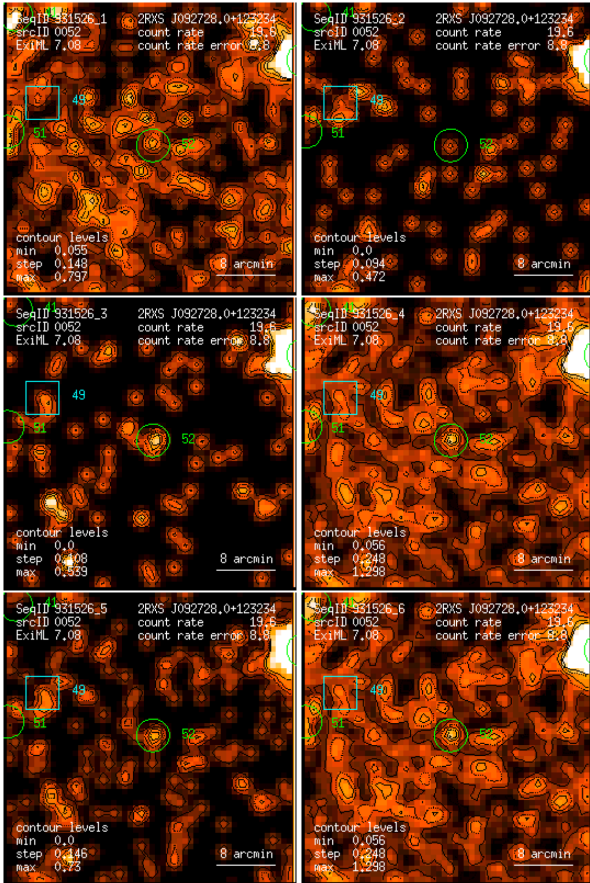
Figure 52: RASS 931526: detection 0052: band rate images, Gaussian filter: (1) PSPC channels 11 – 41, (2) 52 – 90, (3) 91 – 201, (4) 11 – 235, (5) 52 – 201, (6) 11 – 201. Broad band rates in counts/ks. Band rate contour levels in counts/ks/arcmin 2 .
