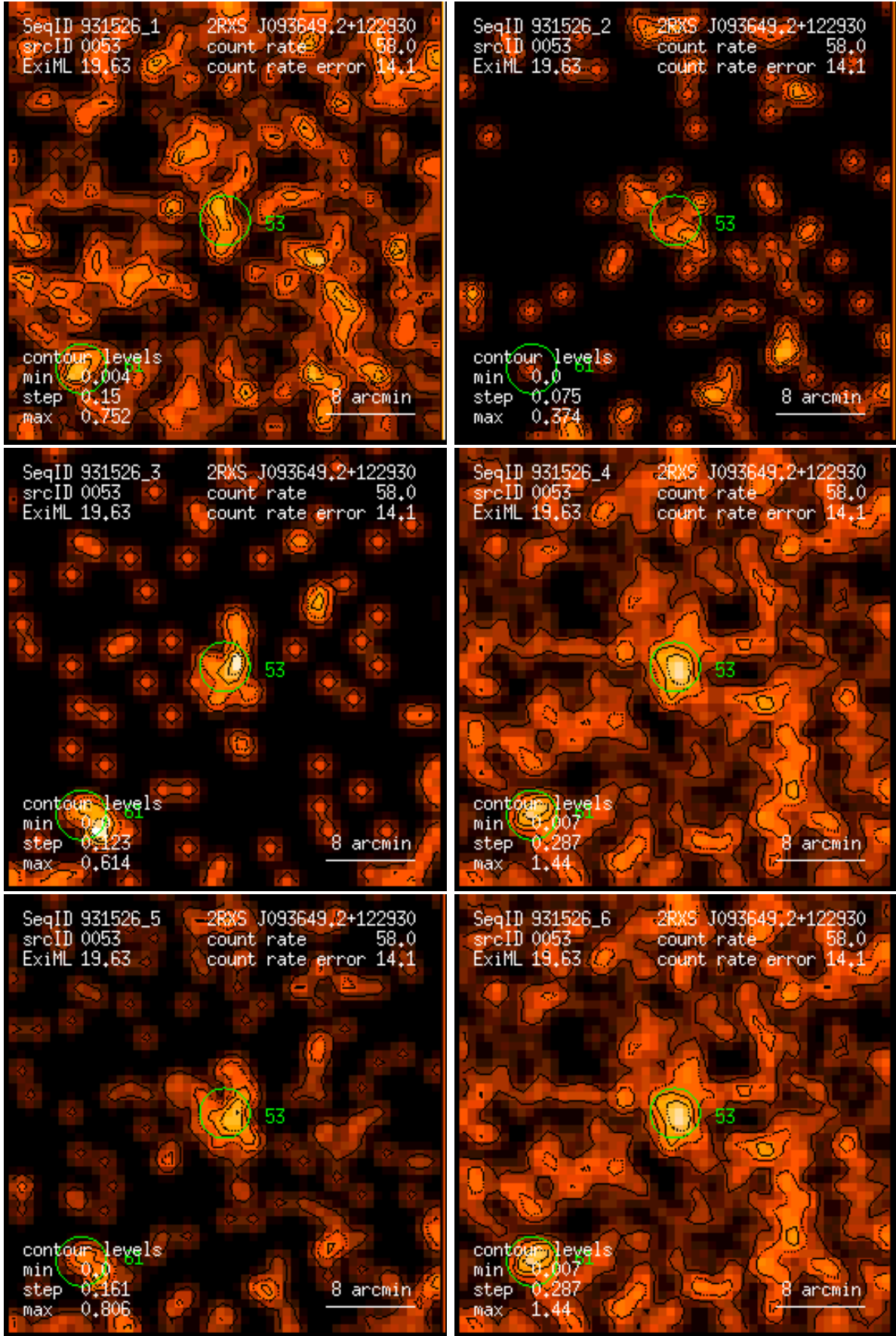
Figure 53: RASS 931526: detection 0053: band rate images, Gaussian filter: (1) PSPC channels 11 – 41, (2) 52 – 90, (3) 91 – 201, (4) 11 – 235, (5) 52 – 201, (6) 11 – 201. Broad band rates in counts/ks. Band rate contour levels in counts/ks/arcmin 2 .
