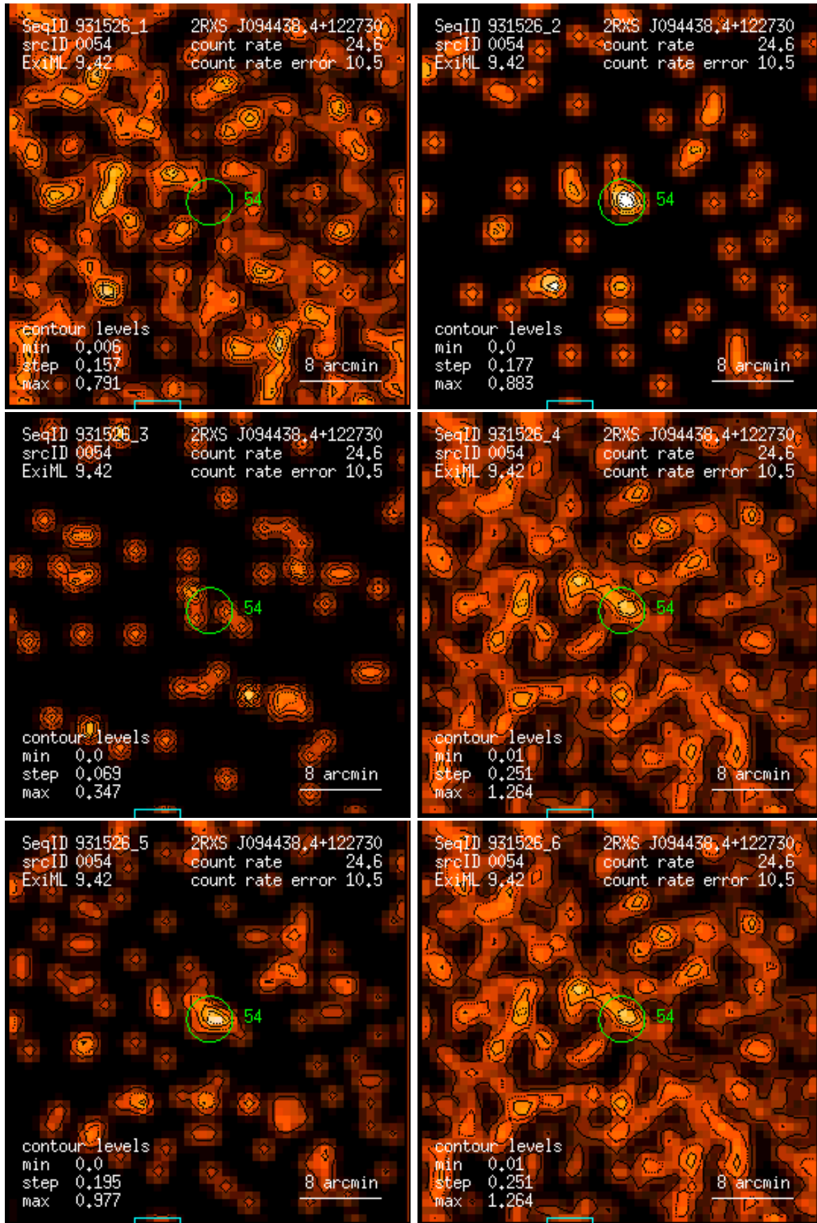
Figure 54: RASS 931526: detection 0054: band rate images, Gaussian filter: (1) PSPC channels 11 – 41, (2) 52 – 90, (3) 91 – 201, (4) 11 – 235, (5) 52 – 201, (6) 11 – 201. Broad band rates in counts/ks. Band rate contour levels in counts/ks/arcmin 2 .
