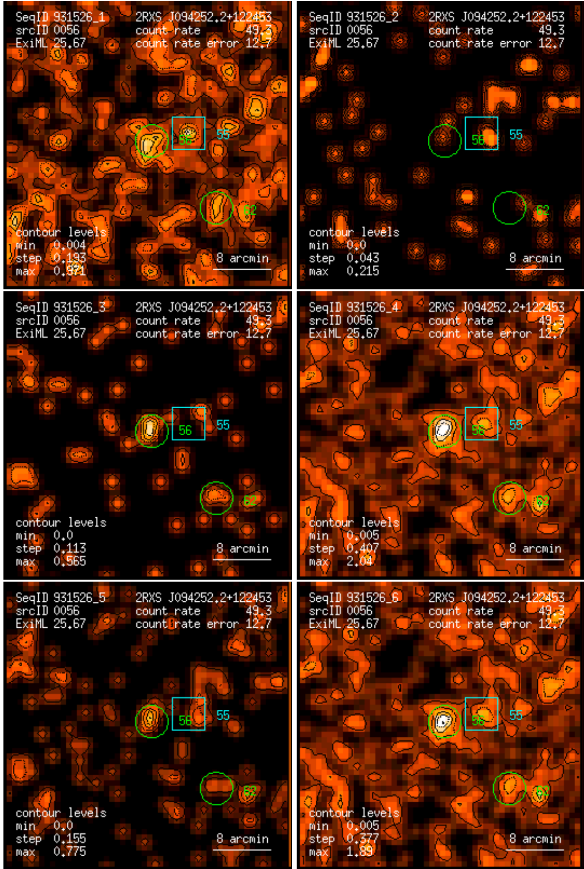
Figure 56: RASS 931526: detection 0056: band rate images, Gaussian filter: (1) PSPC channels 11 – 41, (2) 52 – 90, (3) 91 – 201, (4) 11 – 235, (5) 52 – 201, (6) 11 – 201. Broad band rates in counts/ks. Band rate contour levels in counts/ks/arcmin 2 .
