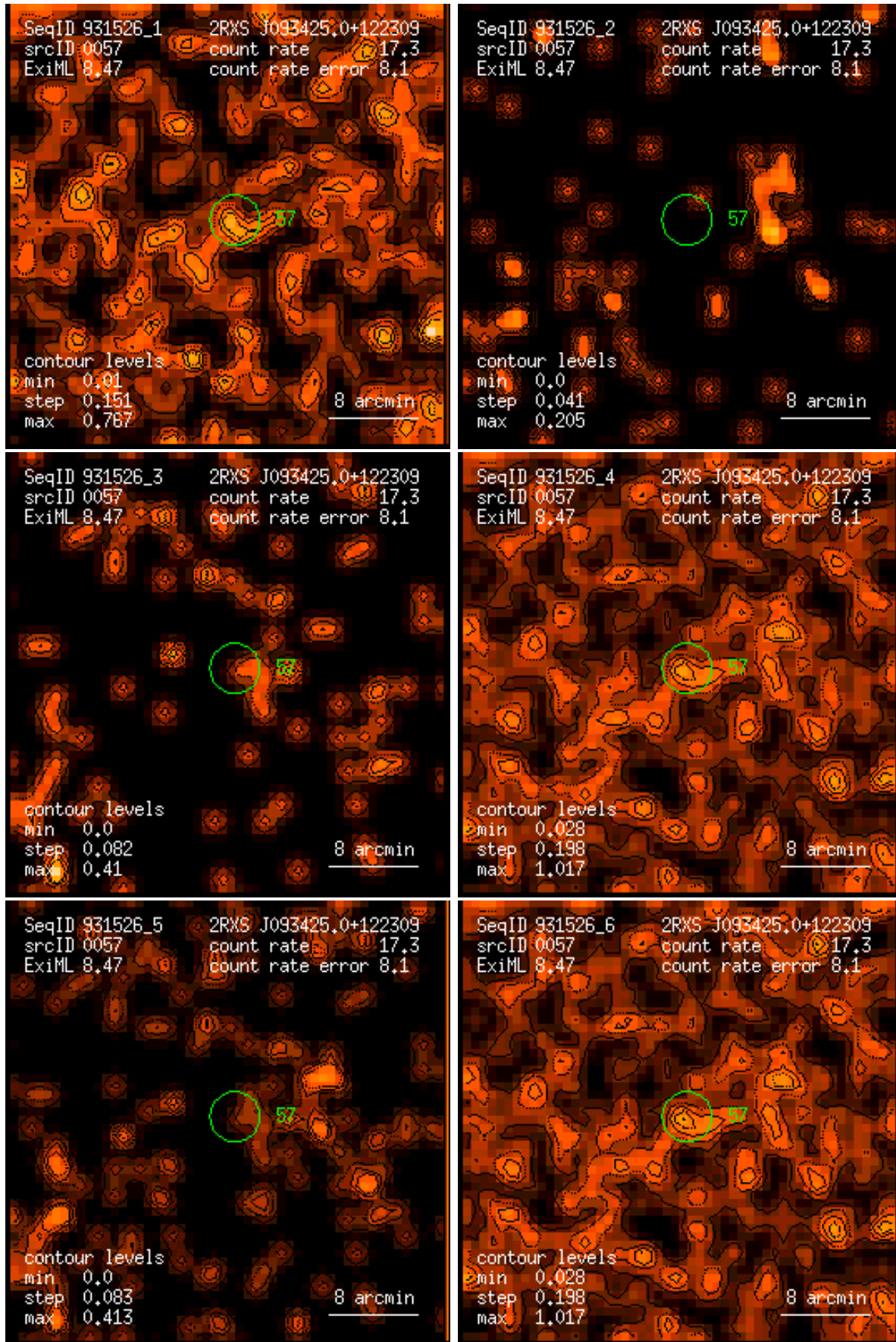
Figure 57: RASS 931526: detection 0057: band rate images, Gaussian filter: (1) PSPC channels 11 – 41, (2) 52 – 90, (3) 91 – 201, (4) 11 – 235, (5) 52 – 201, (6) 11 – 201. Broad band rates in counts/ks. Band rate contour levels in counts/ks/arcmin 2 .
