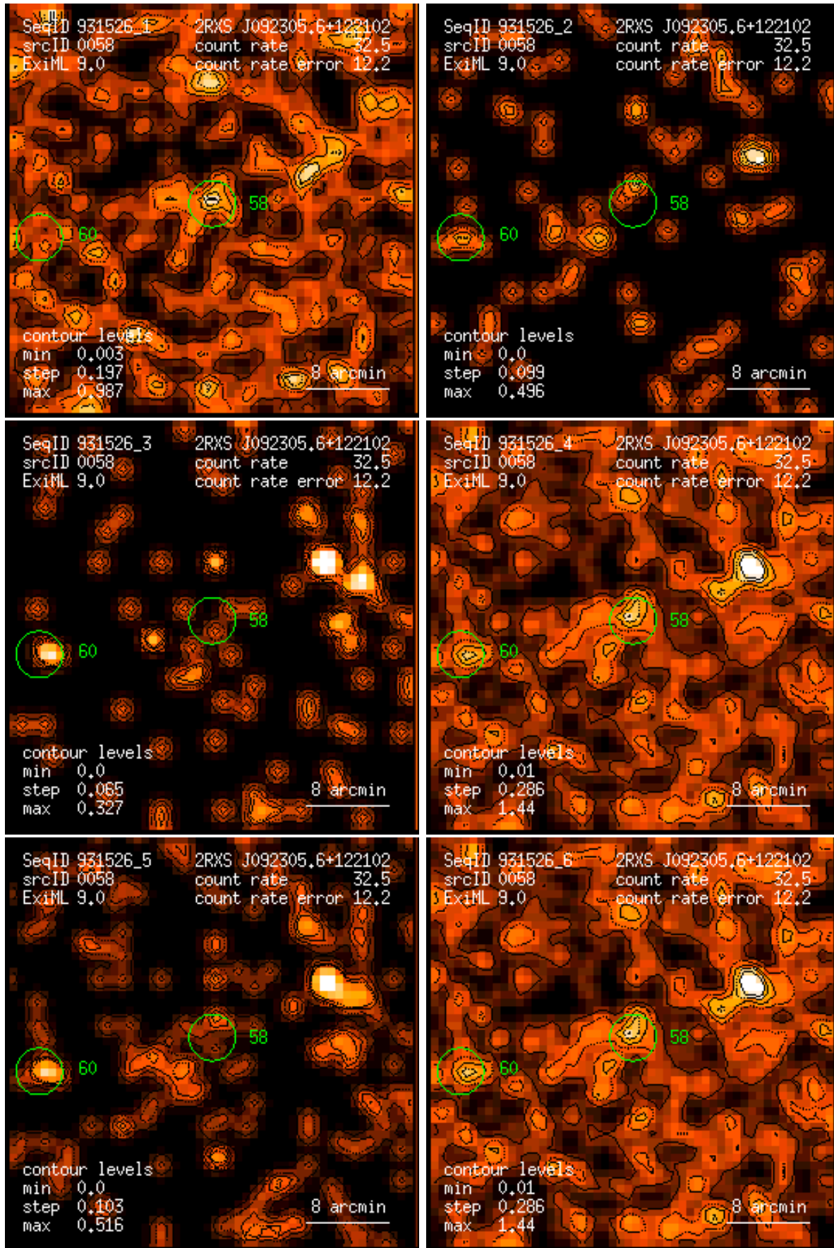
Figure 58: RASS 931526: detection 0058: band rate images, Gaussian filter: (1) PSPC channels 11 – 41, (2) 52 – 90, (3) 91 – 201, (4) 11 – 235, (5) 52 – 201, (6) 11 – 201. Broad band rates in counts/ks. Band rate contour levels in counts/ks/arcmin 2 .
