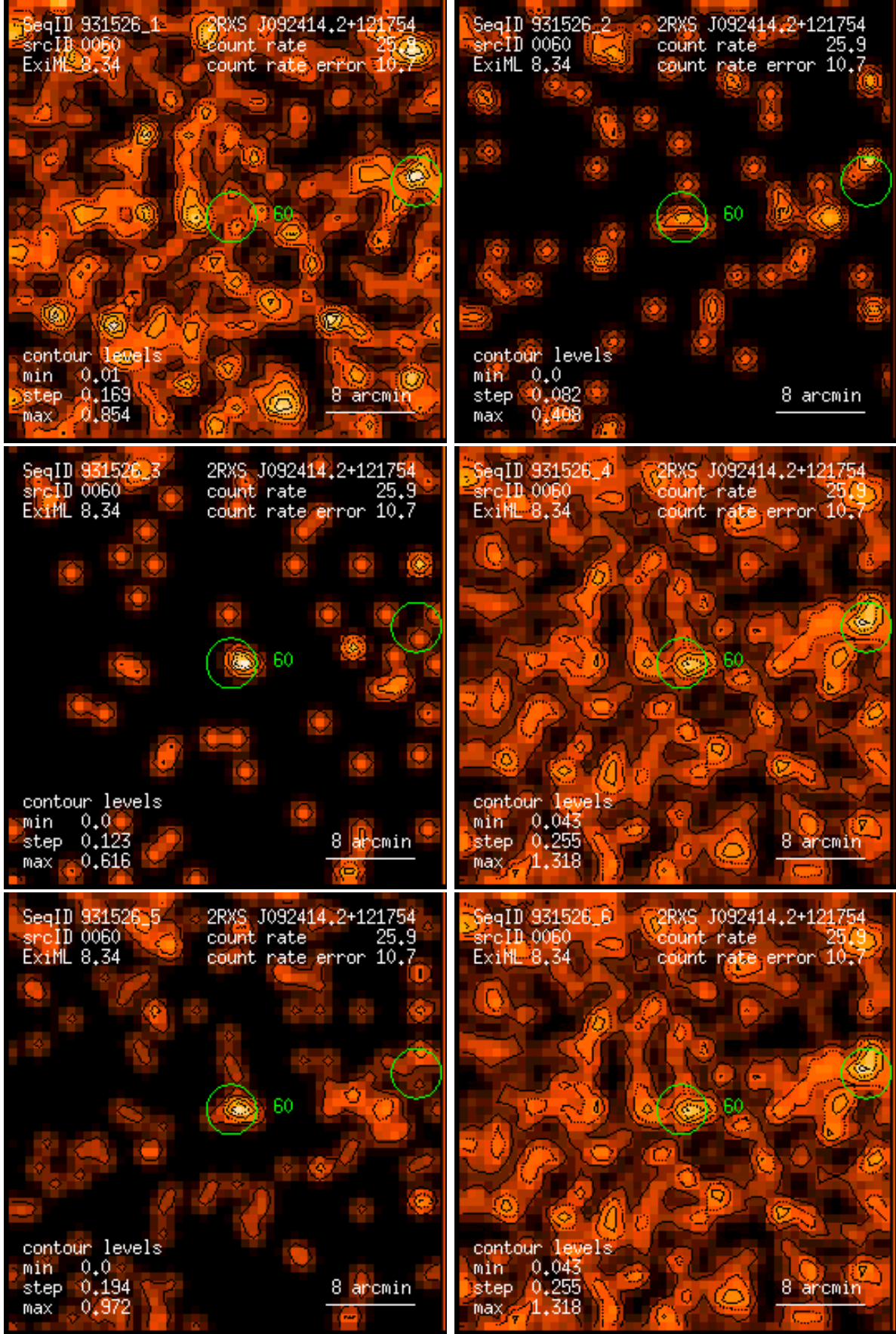
Figure 60: RASS 931526: detection 0060: band rate images, Gaussian filter: (1) PSPC channels 11 – 41, (2) 52 – 90, (3) 91 – 201, (4) 11 – 235, (5) 52 – 201, (6) 11 – 201. Broad band rates in counts/ks. Band rate contour levels in counts/ks/arcmin 2 .
