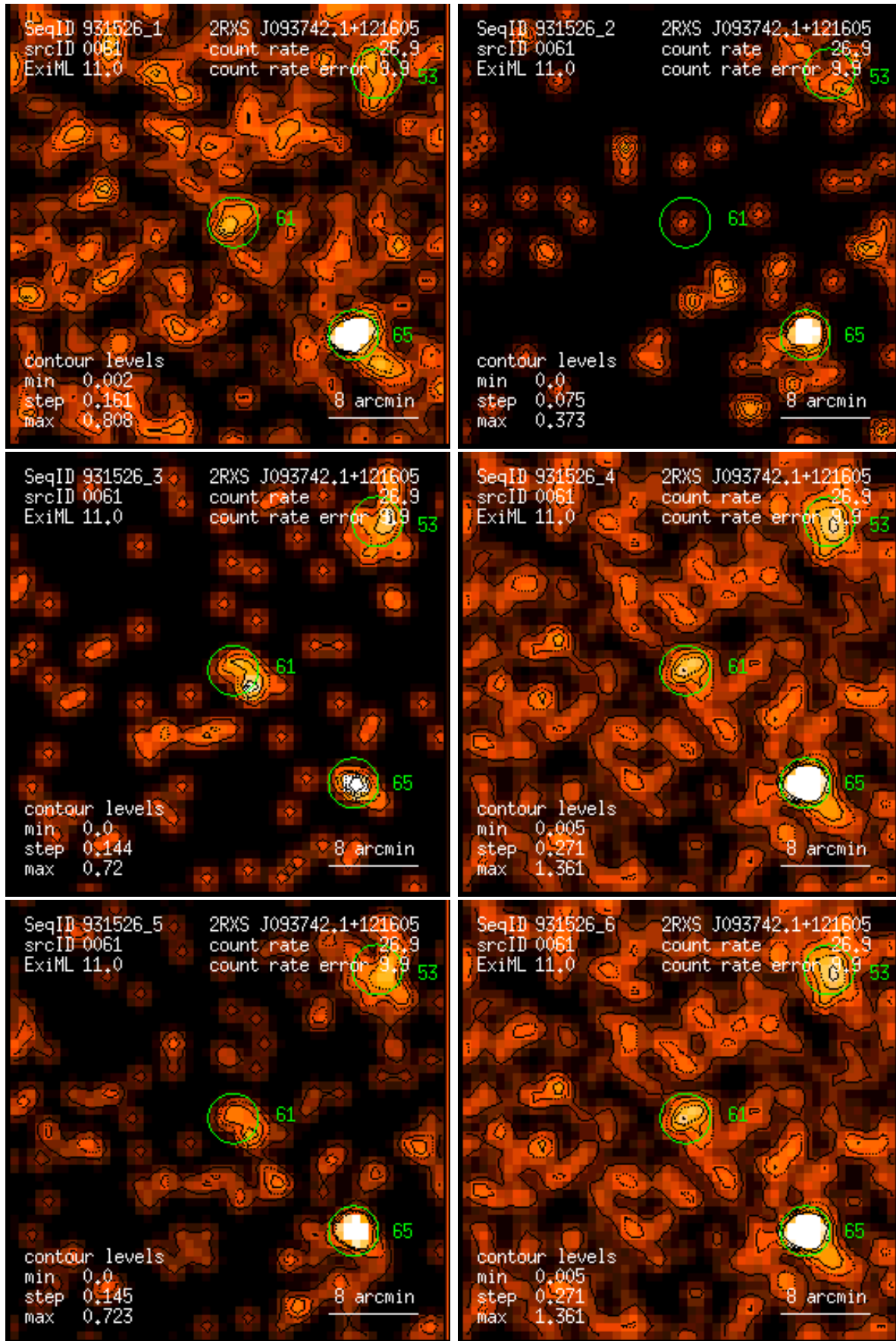
Figure 61: RASS 931526: detection 0061: band rate images, Gaussian filter: (1) PSPC channels 11 – 41, (2) 52 – 90, (3) 91 – 201, (4) 11 – 235, (5) 52 – 201, (6) 11 – 201. Broad band rates in counts/ks. Band rate contour levels in counts/ks/arcmin 2 .
