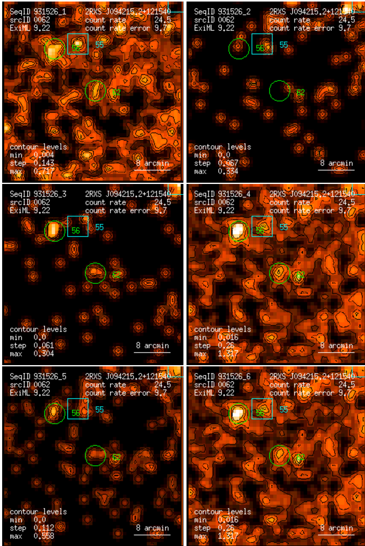
Figure 62: RASS 931526: detection 0062: band rate images, Gaussian filter: (1) PSPC channels 11 – 41, (2) 52 – 90, (3) 91 – 201, (4) 11 – 235, (5) 52 – 201, (6) 11 – 201. Broad band rates in counts/ks. Band rate contour levels in counts/ks/arcmin 2 .
