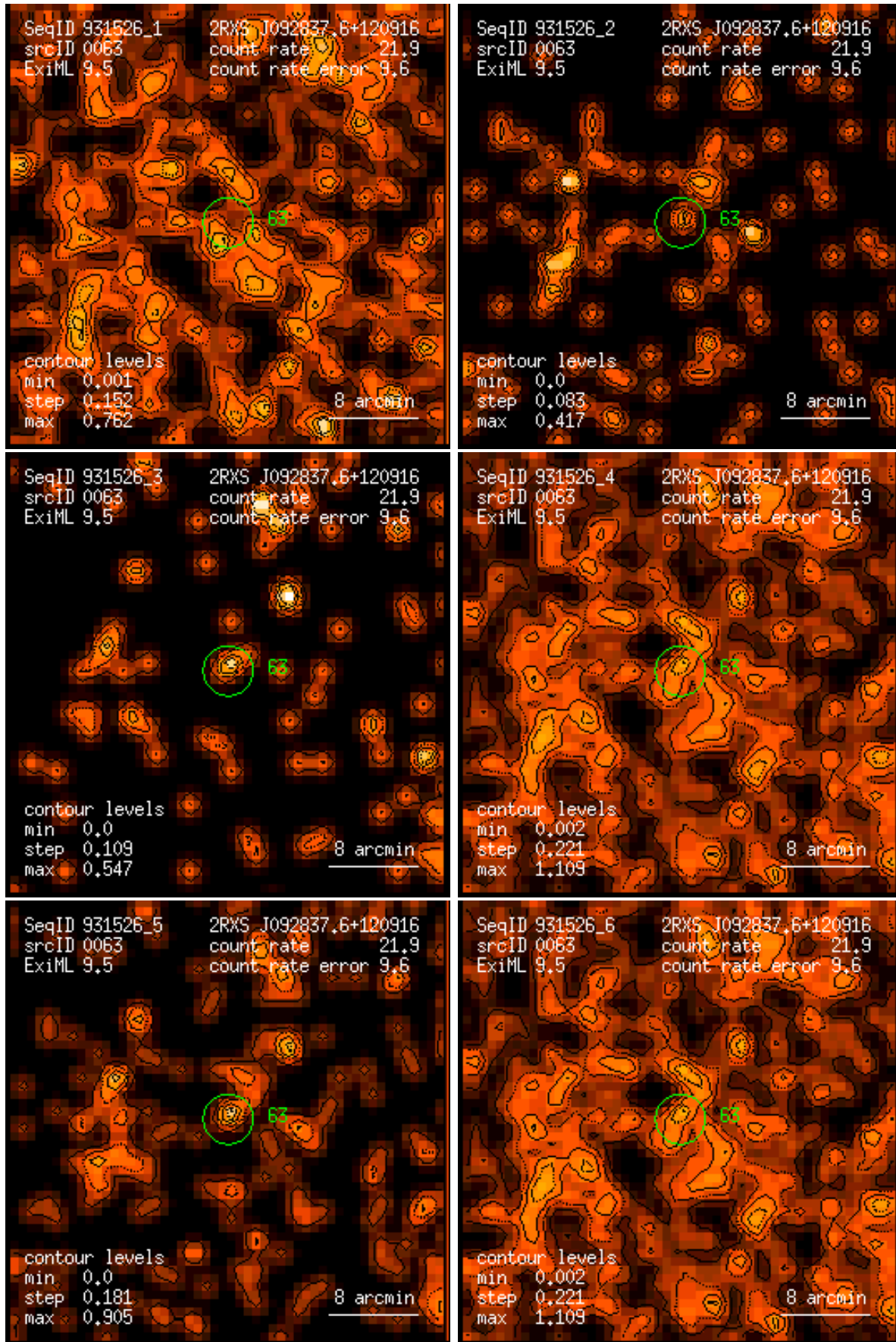
Figure 63: RASS 931526: detection 0063: band rate images, Gaussian filter: (1) PSPC channels 11 – 41, (2) 52 – 90, (3) 91 – 201, (4) 11 – 235, (5) 52 – 201, (6) 11 – 201. Broad band rates in counts/ks. Band rate contour levels in counts/ks/arcmin 2 .
