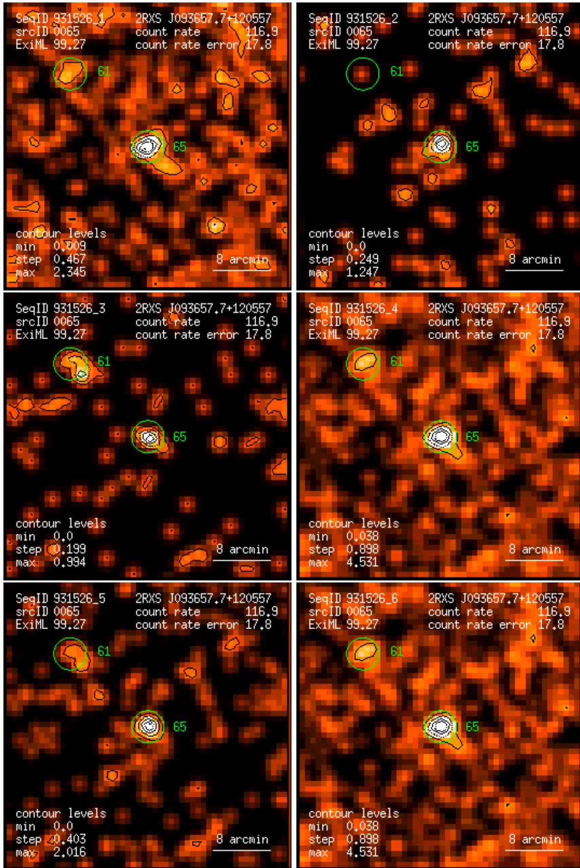
Figure 65: RASS 931526: detection 0065: band rate images, Gaussian filter: (1) PSPC channels 11 – 41, (2) 52 – 90, (3) 91 – 201, (4) 11 – 235, (5) 52 – 201, (6) 11 – 201. Broad band rates in counts/ks. Band rate contour levels in counts/ks/arcmin 2 .
