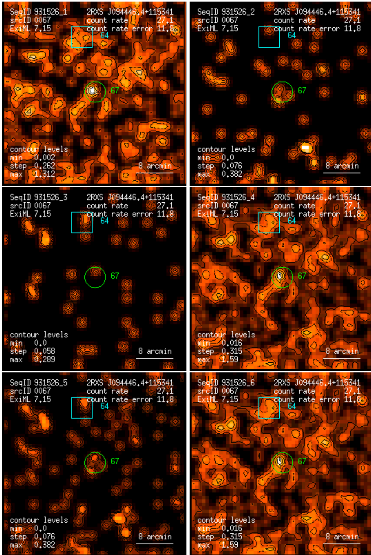
Figure 67: RASS 931526: detection 0067: band rate images, Gaussian filter: (1) PSPC channels 11 – 41, (2) 52 – 90, (3) 91 – 201, (4) 11 – 235, (5) 52 – 201, (6) 11 – 201. Broad band rates in counts/ks. Band rate contour levels in counts/ks/arcmin 2 .
