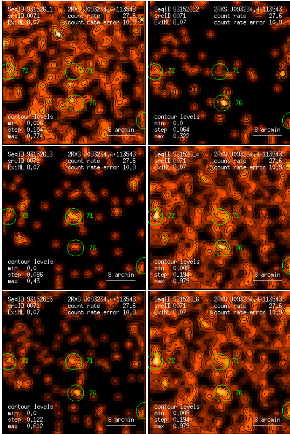
Figure 71: RASS 931526: detection 0071: band rate images, Gaussian filter: (1) PSPC channels 11 – 41, (2) 52 – 90, (3) 91 – 201, (4) 11 – 235, (5) 52 – 201, (6) 11 – 201. Broad band rates in counts/ks. Band rate contour levels in counts/ks/arcmin 2 .
