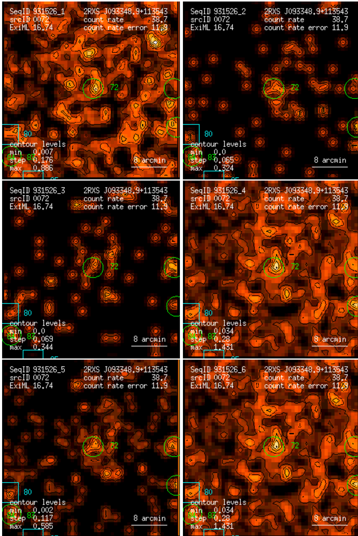
Figure 72: RASS 931526: detection 0072: band rate images, Gaussian filter: (1) PSPC channels 11 – 41, (2) 52 – 90, (3) 91 – 201, (4) 11 – 235, (5) 52 – 201, (6) 11 – 201. Broad band rates in counts/ks. Band rate contour levels in counts/ks/arcmin 2 .
