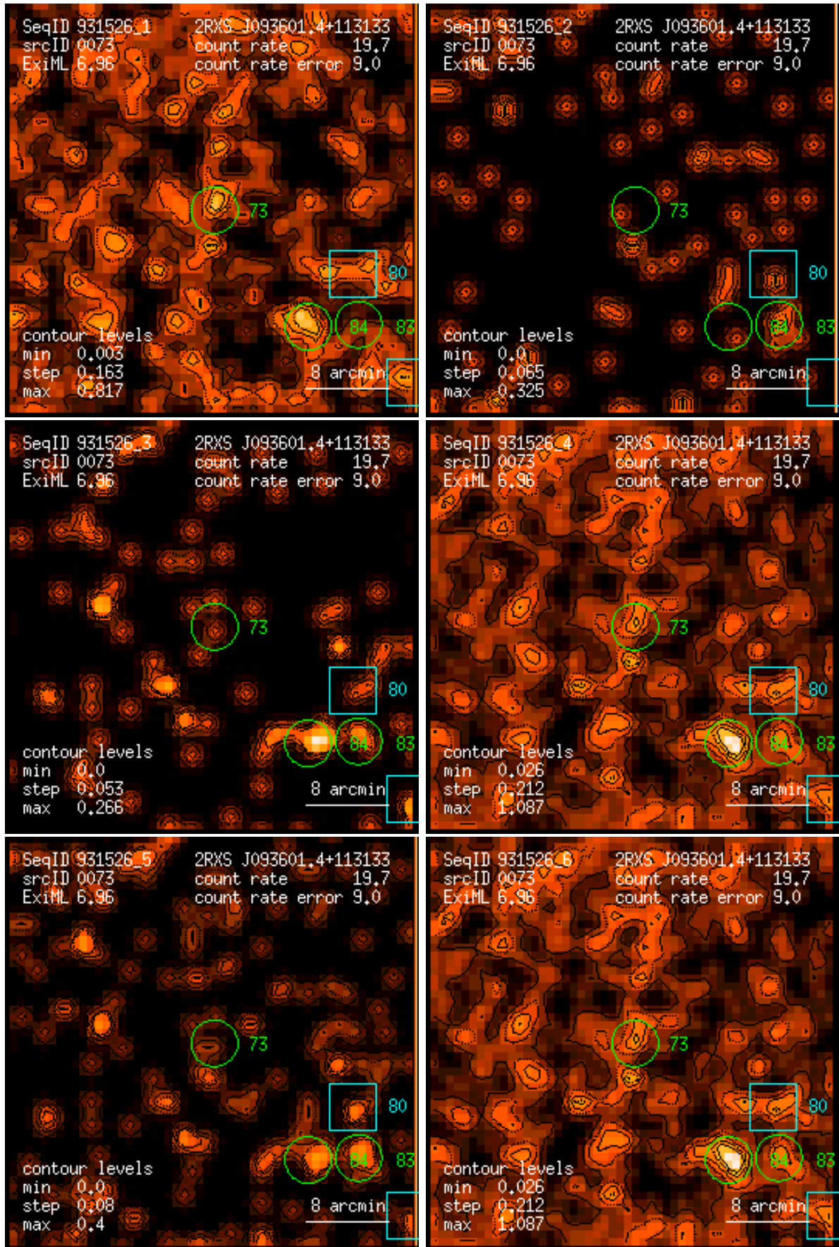
Figure 73: RASS 931526: detection 0073: band rate images, Gaussian filter: (1) PSPC channels 11 – 41, (2) 52 – 90, (3) 91 – 201, (4) 11 – 235, (5) 52 – 201, (6) 11 – 201. Broad band rates in counts/ks. Band rate contour levels in counts/ks/arcmin 2 .
