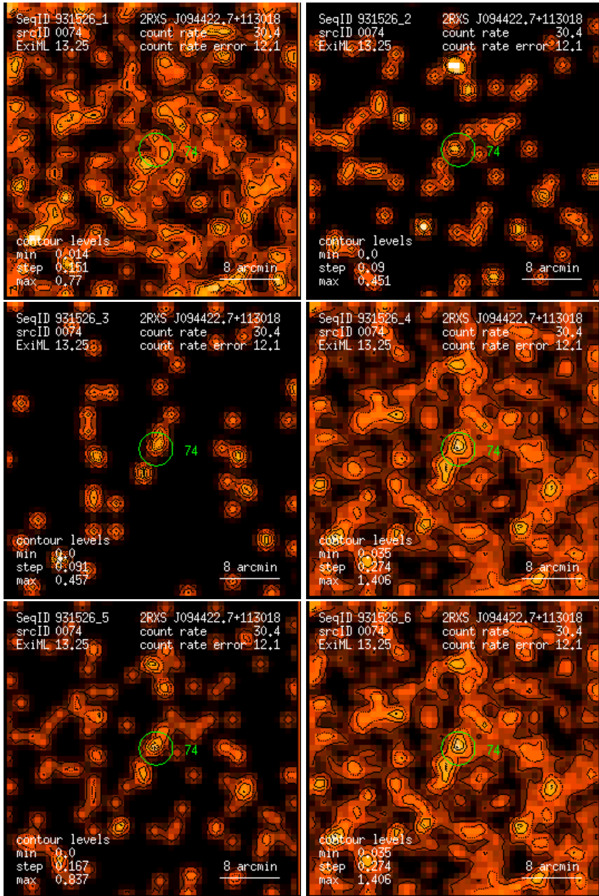
Figure 74: RASS 931526: detection 0074: band rate images, Gaussian filter: (1) PSPC channels 11 – 41, (2) 52 – 90, (3) 91 – 201, (4) 11 – 235, (5) 52 – 201, (6) 11 – 201. Broad band rates in counts/ks. Band rate contour levels in counts/ks/arcmin 2 .
