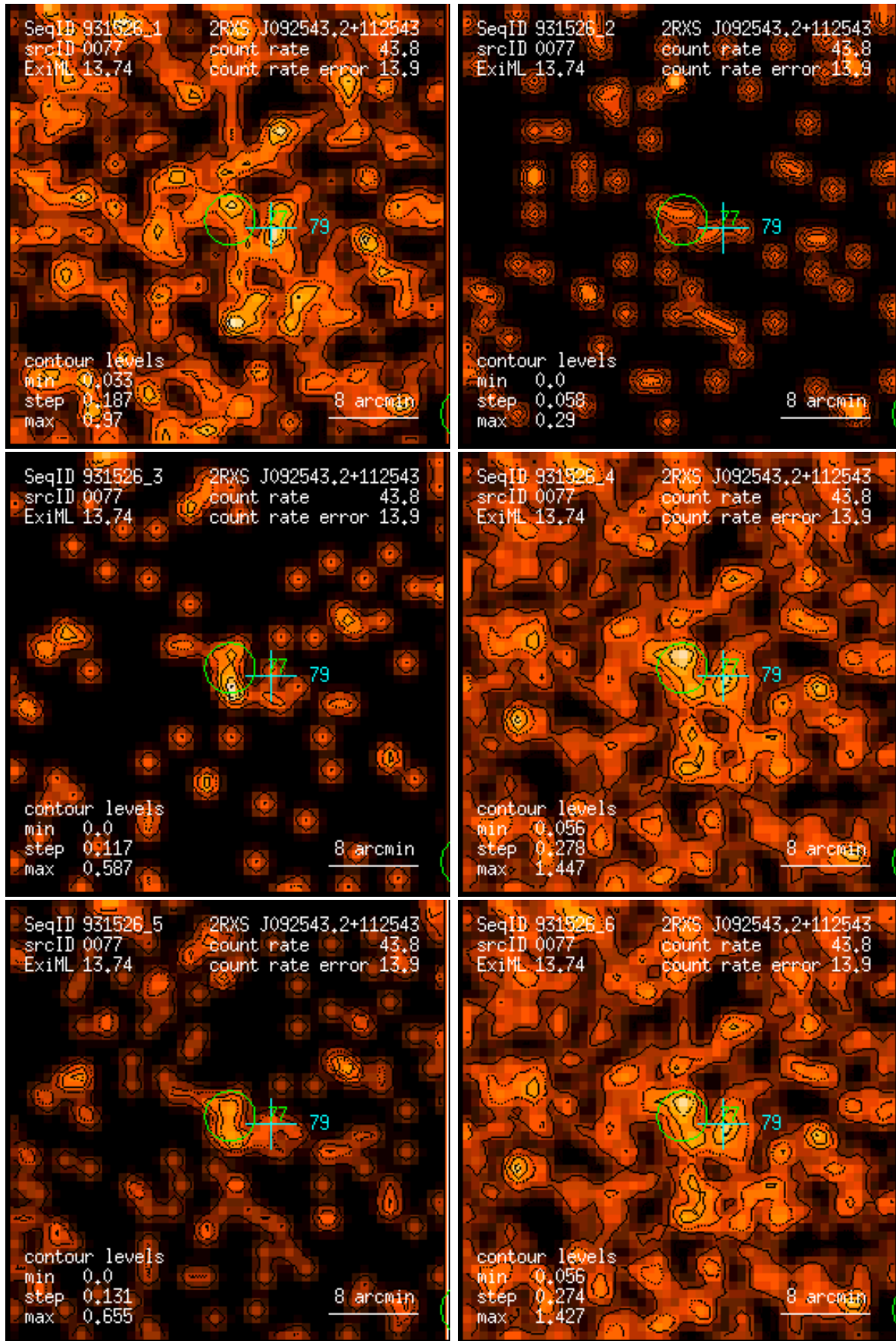
Figure 77: RASS 931526: detection 0077: band rate images, Gaussian filter: (1) PSPC channels 11 – 41, (2) 52 – 90, (3) 91 – 201, (4) 11 – 235, (5) 52 – 201, (6) 11 – 201. Broad band rates in counts/ks. Band rate contour levels in counts/ks/arcmin 2 .
