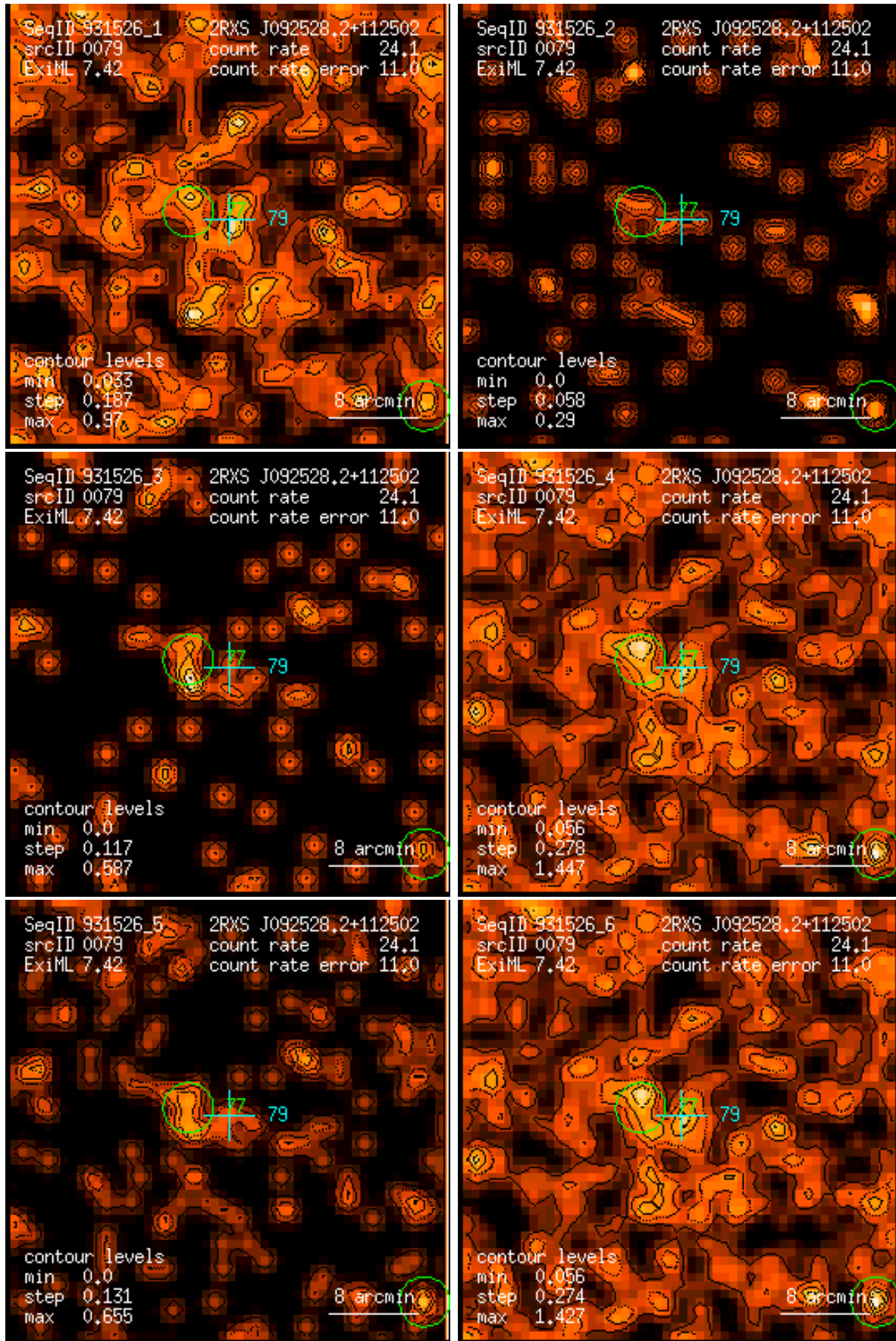
Figure 79: RASS 931526: detection 0079: band rate images, Gaussian filter: (1) PSPC channels 11 – 41, (2) 52 – 90, (3) 91 – 201, (4) 11 – 235, (5) 52 – 201, (6) 11 – 201. Broad band rates in counts/ks. Band rate contour levels in counts/ks/arcmin 2 .
