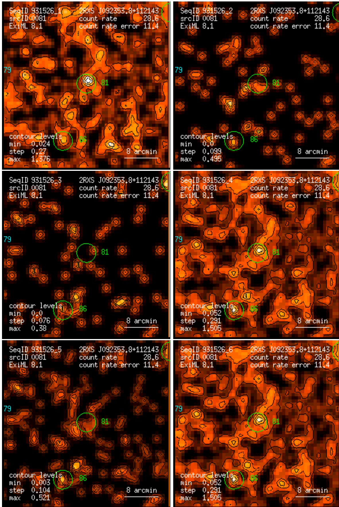
Figure 81: RASS 931526: detection 0081: band rate images, Gaussian filter: (1) PSPC channels 11 – 41, (2) 52 – 90, (3) 91 – 201, (4) 11 – 235, (5) 52 – 201, (6) 11 – 201. Broad band rates in counts/ks. Band rate contour levels in counts/ks/arcmin 2 .
