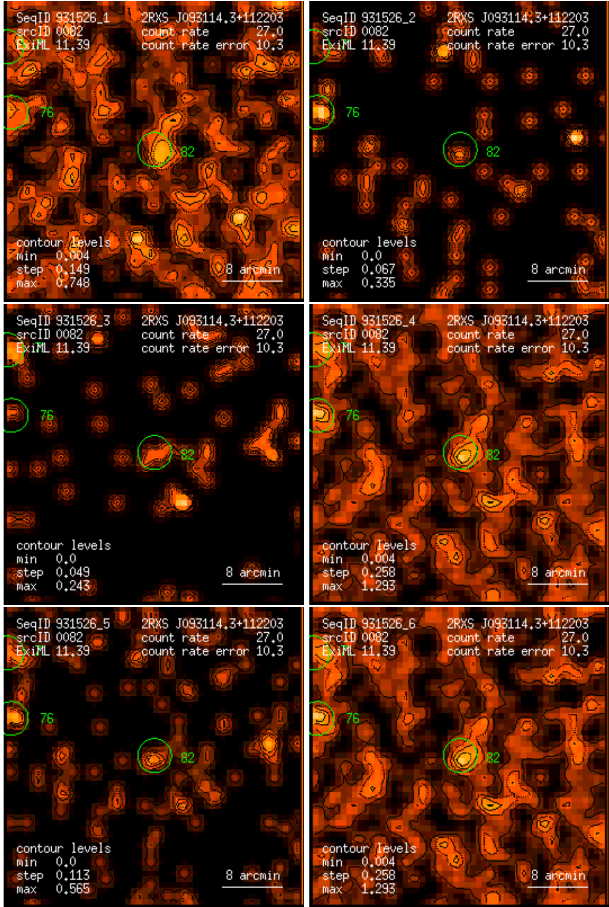
Figure 82: RASS 931526: detection 0082: band rate images, Gaussian filter: (1) PSPC channels 11 – 41, (2) 52 – 90, (3) 91 – 201, (4) 11 – 235, (5) 52 – 201, (6) 11 – 201. Broad band rates in counts/ks. Band rate contour levels in counts/ks/arcmin 2 .
