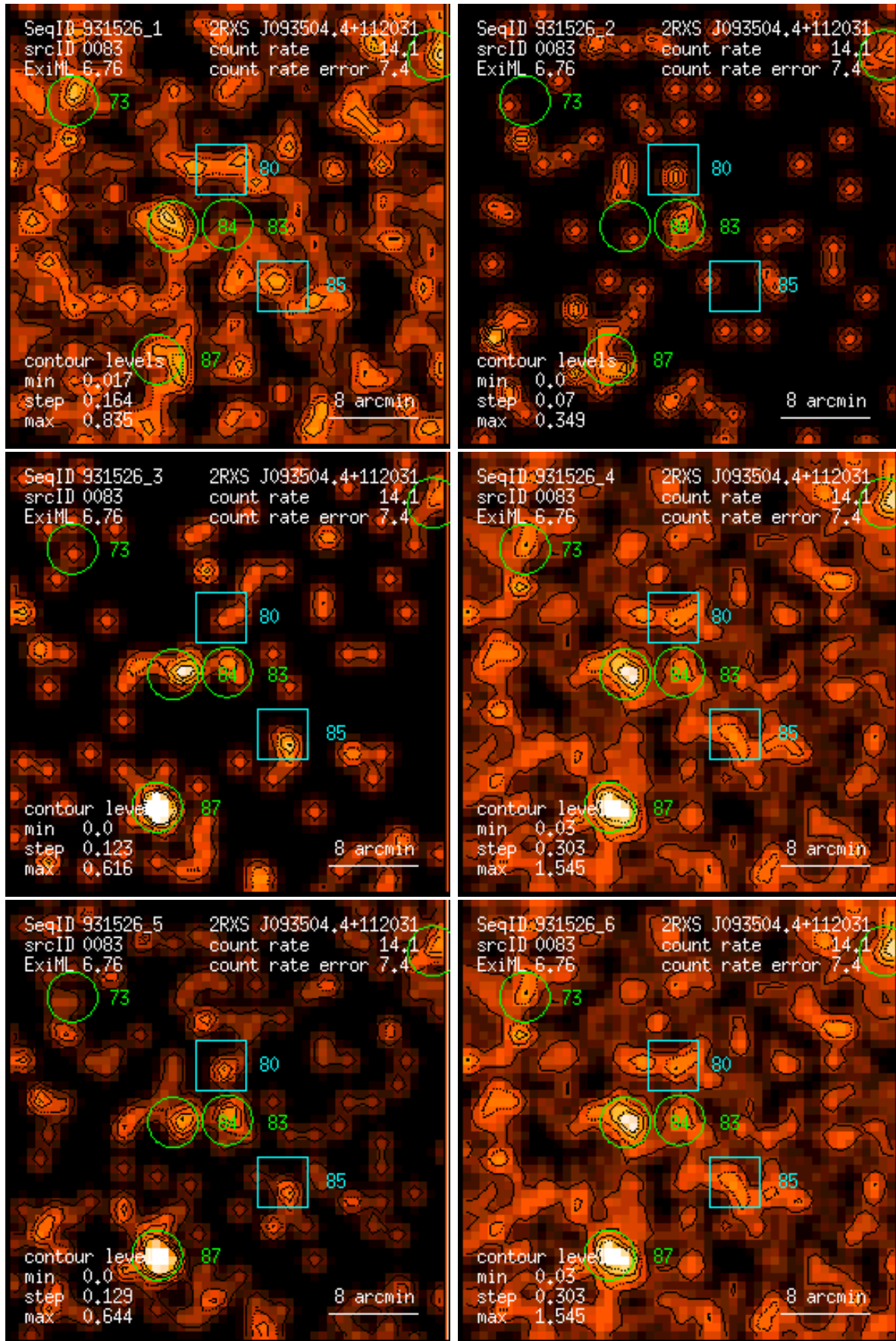
Figure 83: RASS 931526: detection 0083: band rate images, Gaussian filter: (1) PSPC channels 11 – 41, (2) 52 – 90, (3) 91 – 201, (4) 11 – 235, (5) 52 – 201, (6) 11 – 201. Broad band rates in counts/ks. Band rate contour levels in counts/ks/arcmin 2 .
