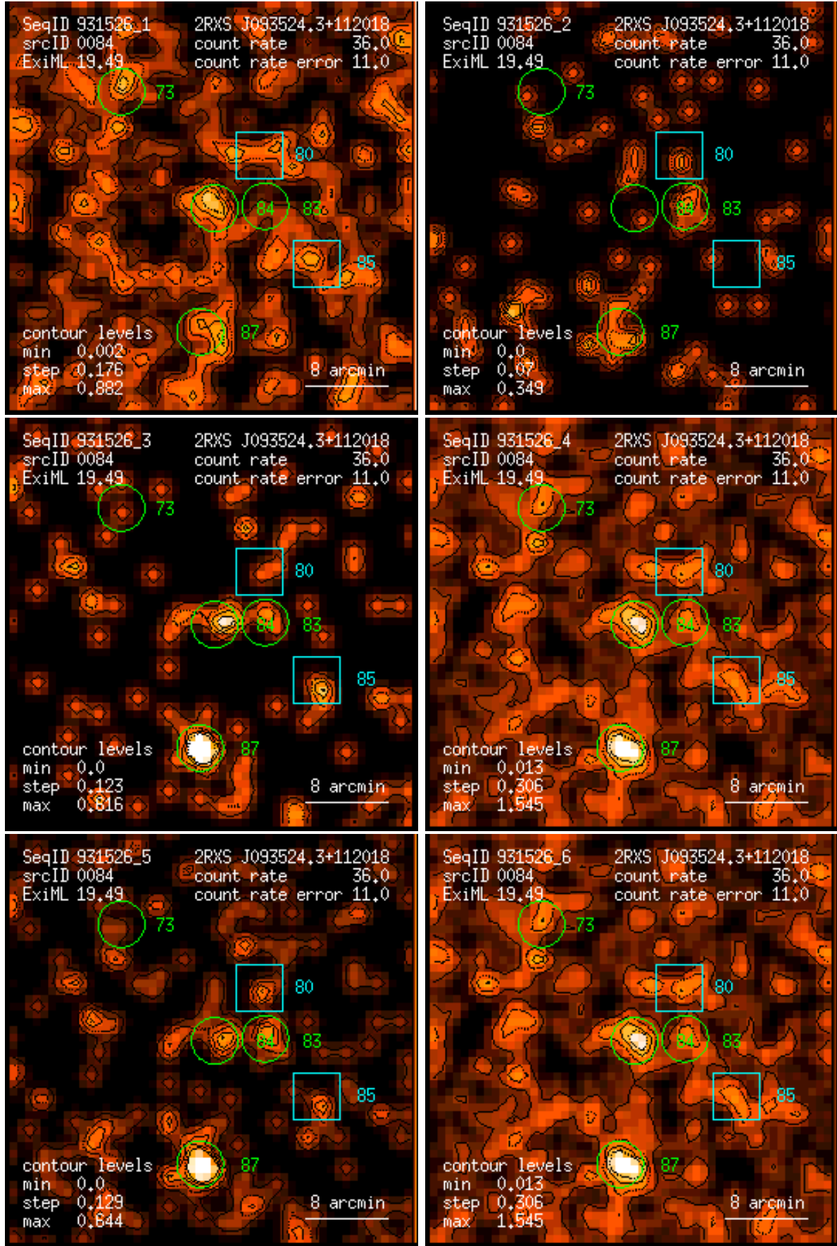
Figure 84: RASS 931526: detection 0084: band rate images, Gaussian filter: (1) PSPC channels 11 – 41, (2) 52 – 90, (3) 91 – 201, (4) 11 – 235, (5) 52 – 201, (6) 11 – 201. Broad band rates in counts/ks. Band rate contour levels in counts/ks/arcmin 2 .
