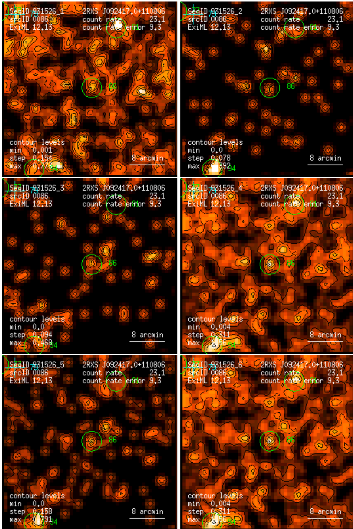
Figure 86: RASS 931526: detection 0086: band rate images, Gaussian filter: (1) PSPC channels 11 – 41, (2) 52 – 90, (3) 91 – 201, (4) 11 – 235, (5) 52 – 201, (6) 11 – 201. Broad band rates in counts/ks. Band rate contour levels in counts/ks/arcmin 2 .
