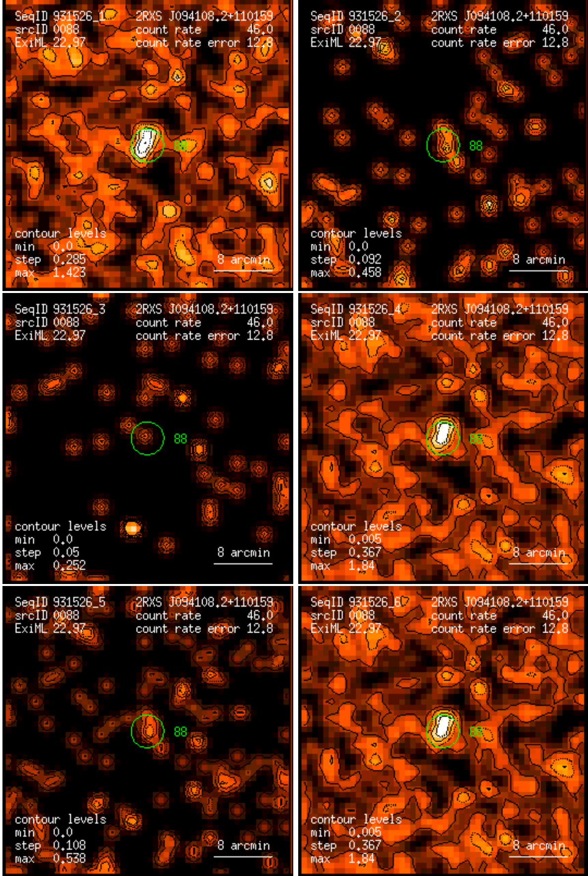
Figure 88: RASS 931526: detection 0088: band rate images, Gaussian filter: (1) PSPC channels 11 – 41, (2) 52 – 90, (3) 91 – 201, (4) 11 – 235, (5) 52 – 201, (6) 11 – 201. Broad band rates in counts/ks. Band rate contour levels in counts/ks/arcmin 2 .
