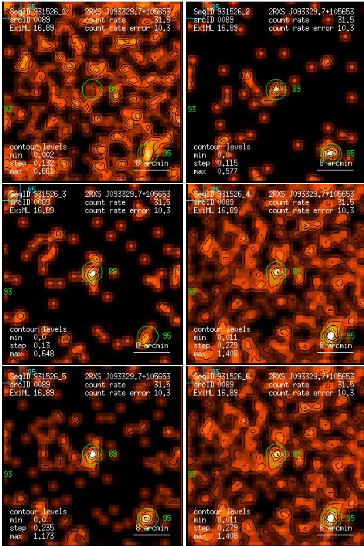
Figure 89: RASS 931526: detection 0089: band rate images, Gaussian filter: (1) PSPC channels 11 – 41, (2) 52 – 90, (3) 91 – 201, (4) 11 – 235, (5) 52 – 201, (6) 11 – 201. Broad band rates in counts/ks. Band rate contour levels in counts/ks/arcmin 2 .
