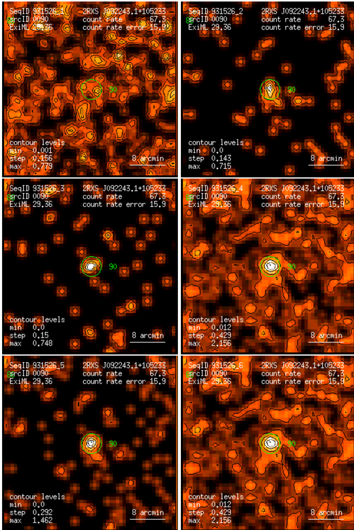
Figure 90: RASS 931526: detection 0090: band rate images, Gaussian filter: (1) PSPC channels 11 – 41, (2) 52 – 90, (3) 91 – 201, (4) 11 – 235, (5) 52 – 201, (6) 11 – 201. Broad band rates in counts/ks. Band rate contour levels in counts/ks/arcmin 2 .
