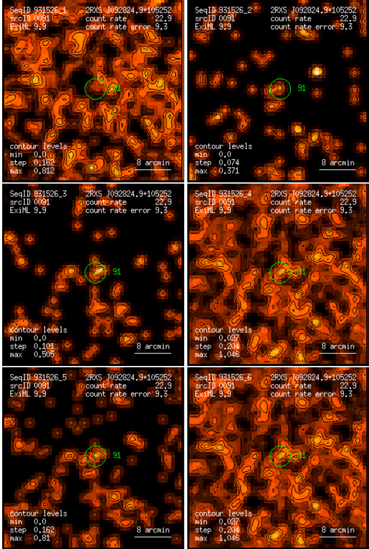
Figure 91: RASS 931526: detection 0091: band rate images, Gaussian filter: (1) PSPC channels 11 – 41, (2) 52 – 90, (3) 91 – 201, (4) 11 – 235, (5) 52 – 201, (6) 11 – 201. Broad band rates in counts/ks. Band rate contour levels in counts/ks/arcmin 2 .
